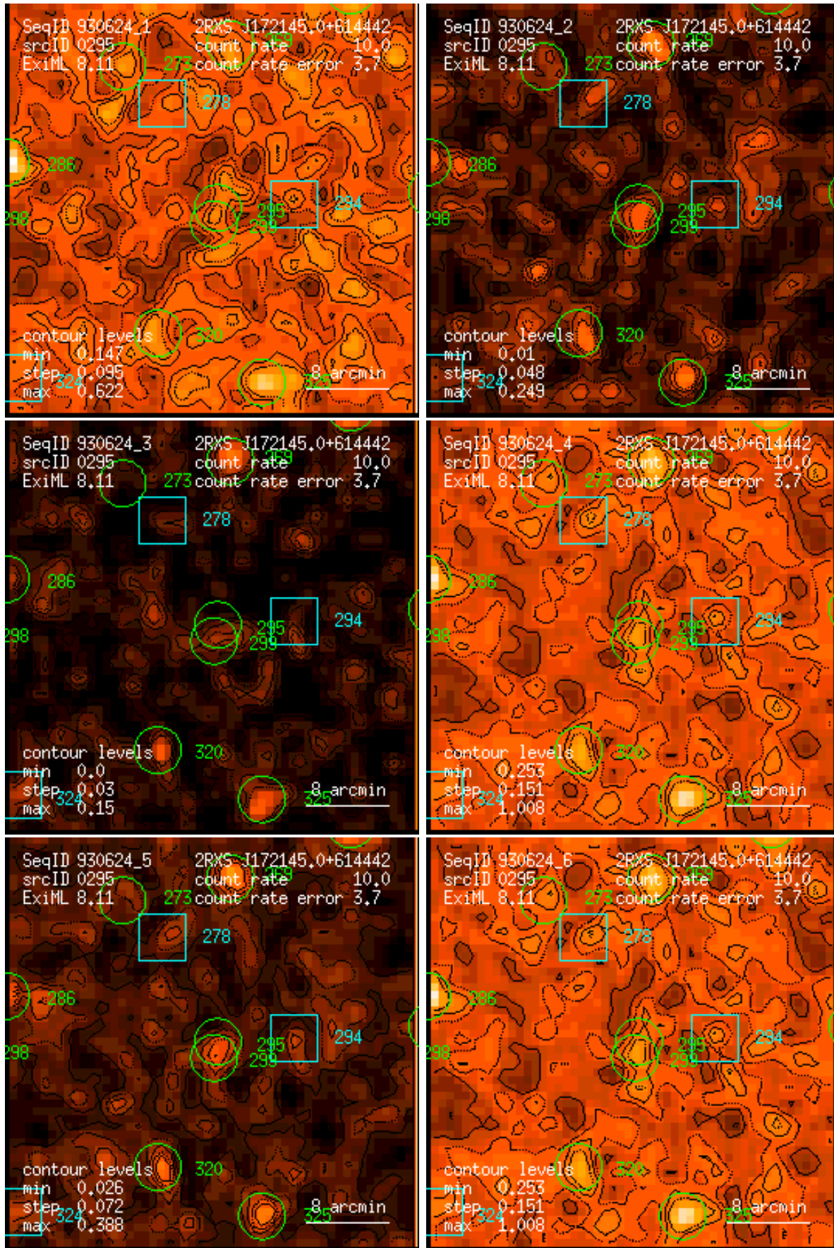
Figure 295: RASS 930624: detection 0295: band rate images, Gaussian filter: (1) PSPC channels 11 – 41, (2) 52 – 90, (3) 91 – 201, (4) 11 – 235, (5) 52 – 201, (6) 11 – 201. Broad band rates in counts/ks. Band rate contour levels in counts/ks/arcmin 2 .
