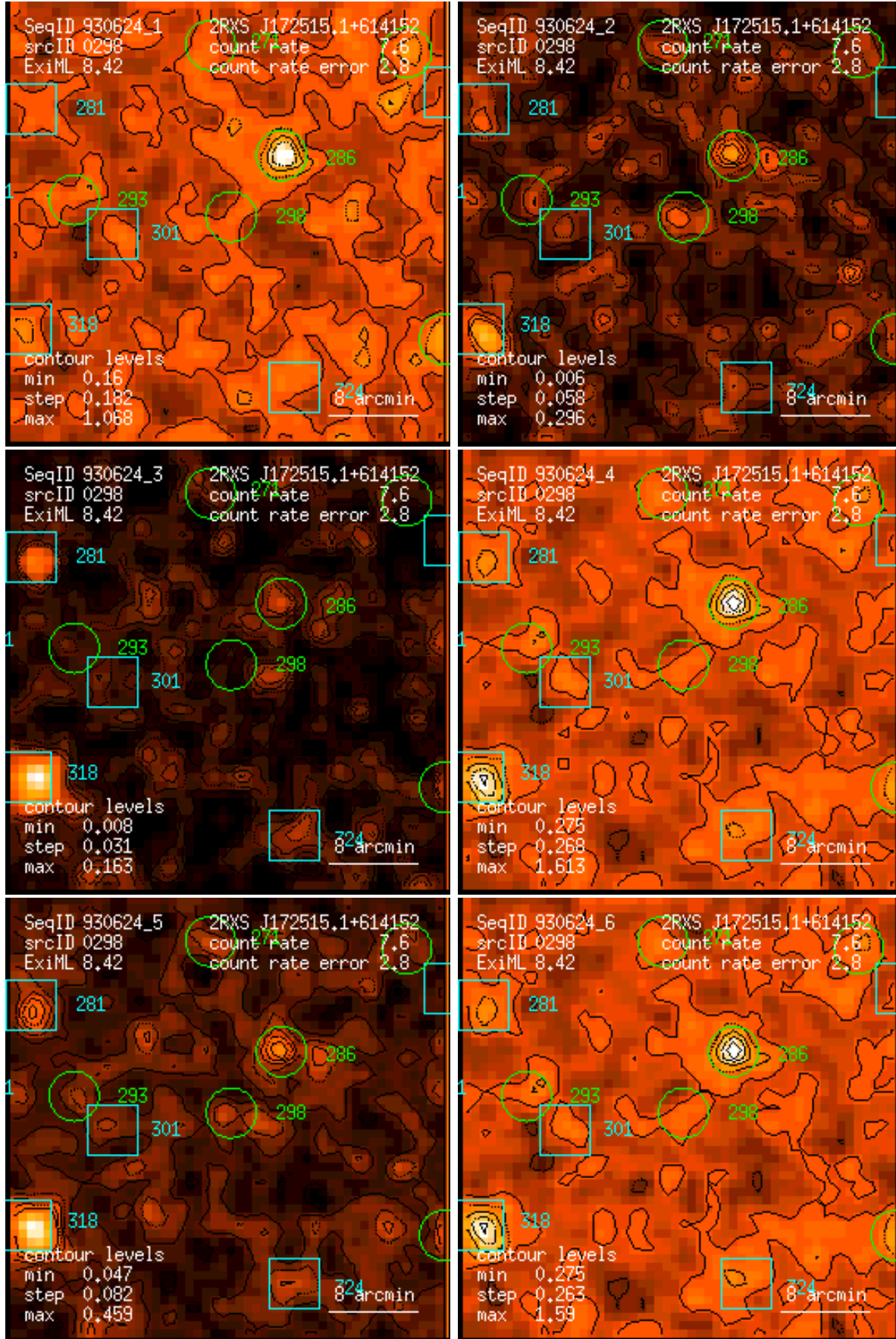
Figure 298: RASS 930624: detection 0298: band rate images, Gaussian filter: (1) PSPC channels 11 – 41, (2) 52 – 90, (3) 91 – 201, (4) 11 – 235, (5) 52 – 201, (6) 11 – 201. Broad band rates in counts/ks. Band rate contour levels in counts/ks/arcmin 2 .
