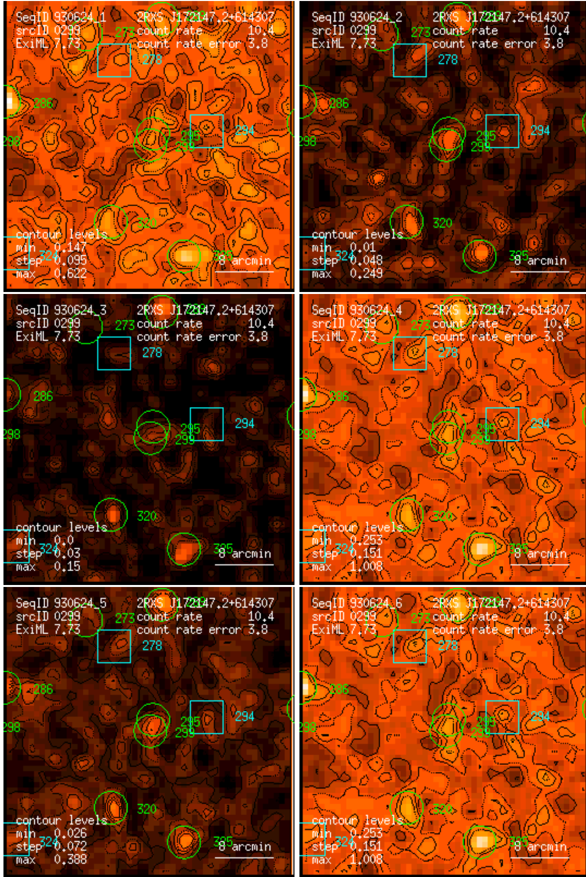
Figure 299: RASS 930624: detection 0299: band rate images, Gaussian filter: (1) PSPC channels 11 – 41, (2) 52 – 90, (3) 91 – 201, (4) 11 – 235, (5) 52 – 201, (6) 11 – 201. Broad band rates in counts/ks. Band rate contour levels in counts/ks/arcmin 2 .
