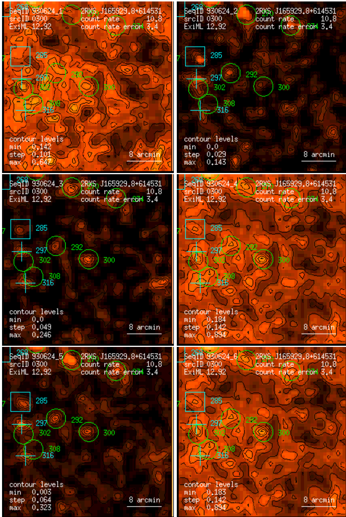
Figure 300: RASS 930624: detection 0300: band rate images, Gaussian filter: (1) PSPC channels 11 – 41, (2) 52 – 90, (3) 91 – 201, (4) 11 – 235, (5) 52 – 201, (6) 11 – 201. Broad band rates in counts/ks. Band rate contour levels in counts/ks/arcmin 2 .
