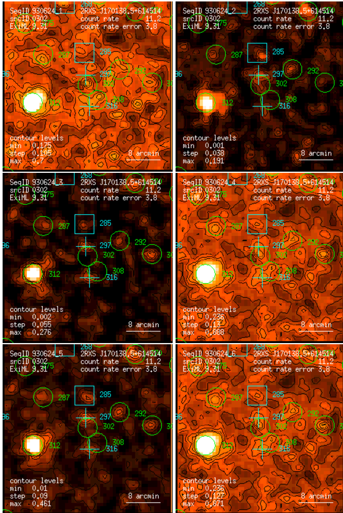
Figure 302: RASS 930624: detection 0302: band rate images, Gaussian filter: (1) PSPC channels 11 – 41, (2) 52 – 90, (3) 91 – 201, (4) 11 – 235, (5) 52 – 201, (6) 11 – 201. Broad band rates in counts/ks. Band rate contour levels in counts/ks/arcmin 2 .
