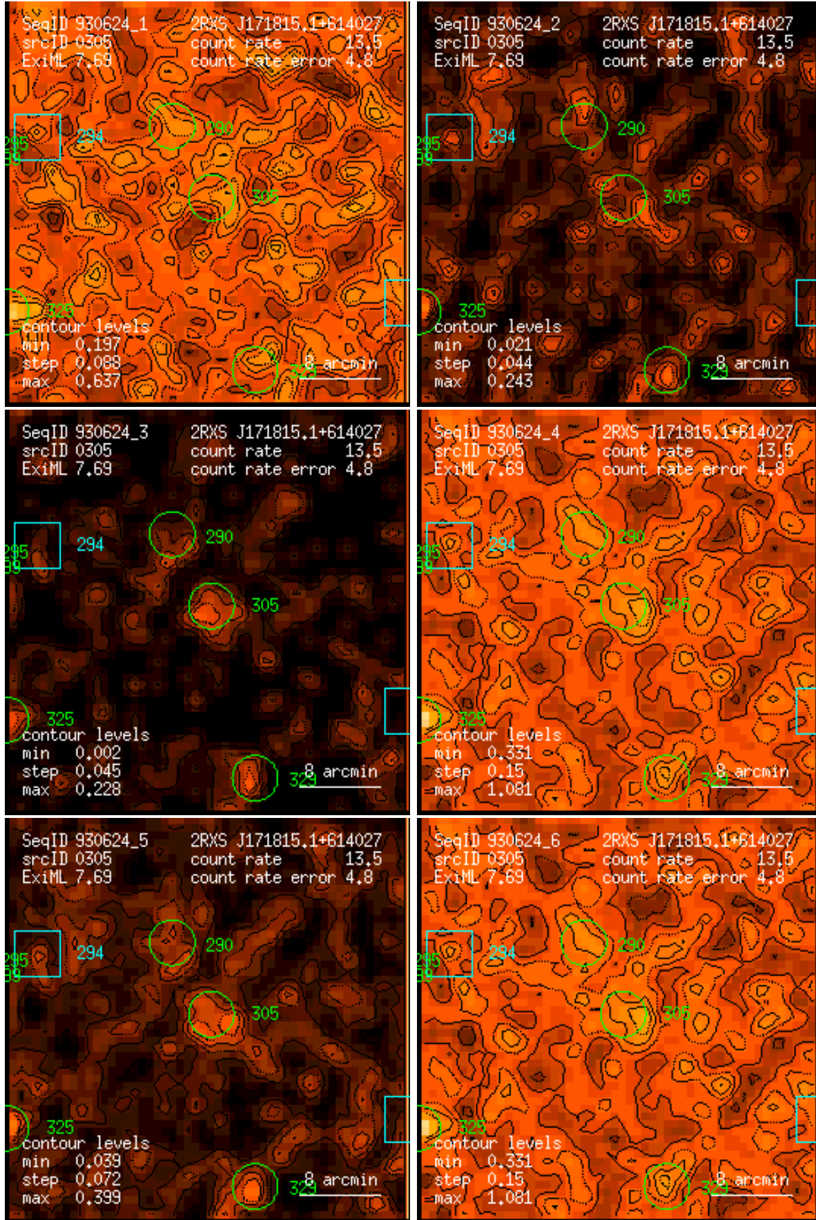
Figure 305: RASS 930624: detection 0305: band rate images, Gaussian filter: (1) PSPC channels 11 – 41, (2) 52 – 90, (3) 91 – 201, (4) 11 – 235, (5) 52 – 201, (6) 11 – 201. Broad band rates in counts/ks. Band rate contour levels in counts/ks/arcmin 2 .
