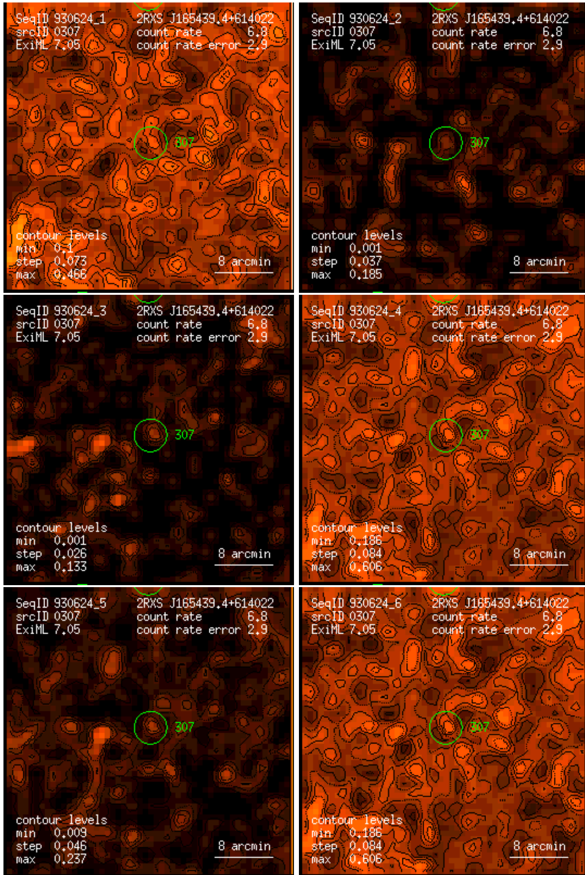
Figure 307: RASS 930624: detection 0307: band rate images, Gaussian filter: (1) PSPC channels 11 – 41, (2) 52 – 90, (3) 91 – 201, (4) 11 – 235, (5) 52 – 201, (6) 11 – 201. Broad band rates in counts/ks. Band rate contour levels in counts/ks/arcmin 2 .
