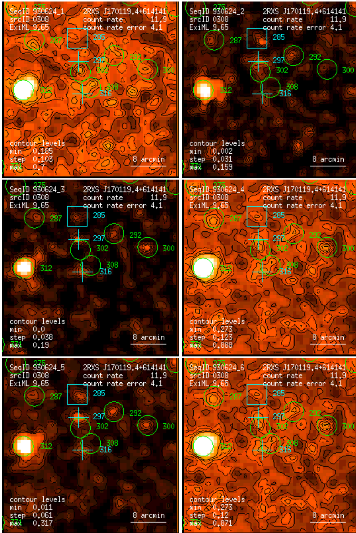
Figure 308: RASS 930624: detection 0308: band rate images, Gaussian filter: (1) PSPC channels 11 – 41, (2) 52 – 90, (3) 91 – 201, (4) 11 – 235, (5) 52 – 201, (6) 11 – 201. Broad band rates in counts/ks. Band rate contour levels in counts/ks/arcmin 2 .
