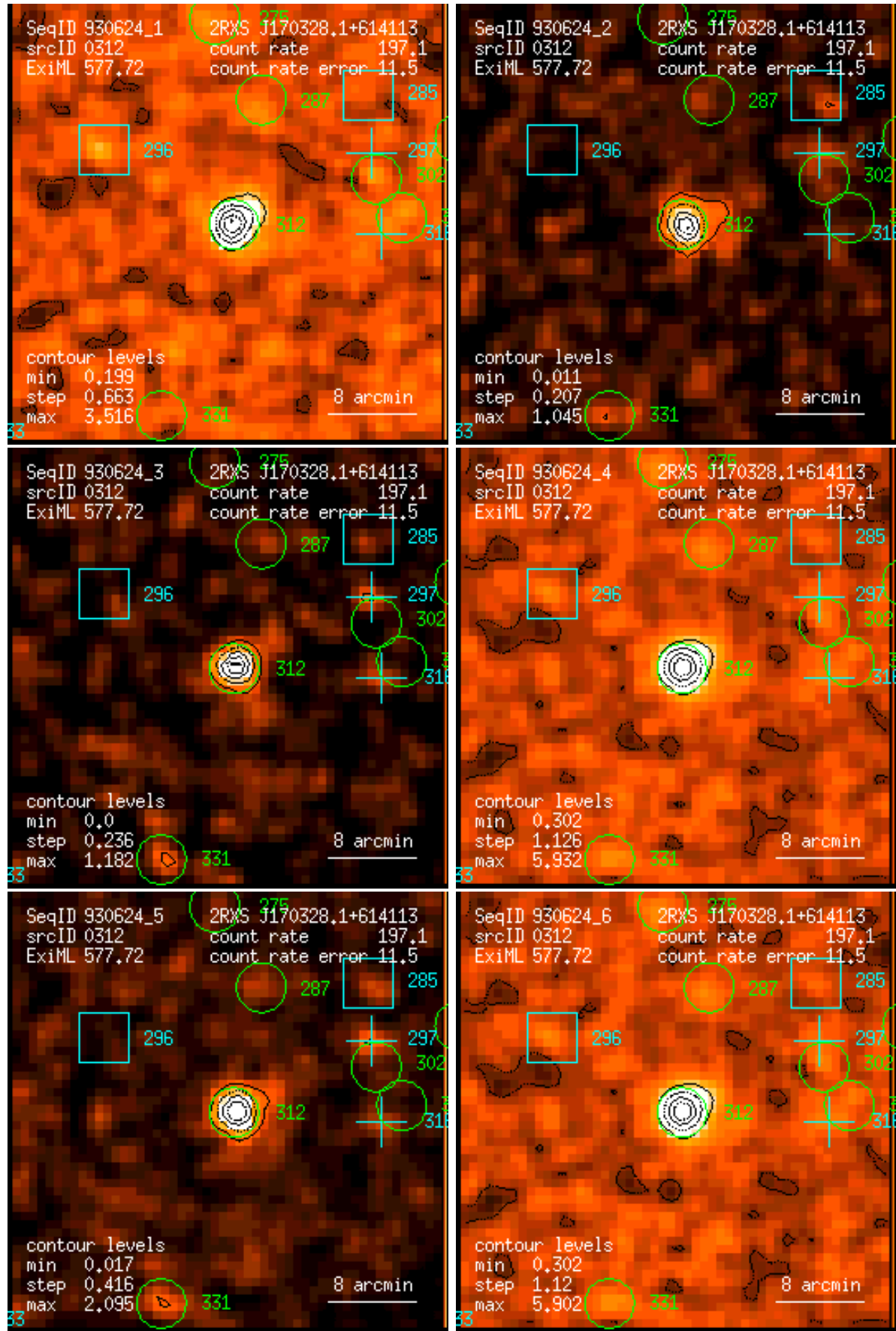
Figure 312: RASS 930624: detection 0312: band rate images, Gaussian filter: (1) PSPC channels 11 – 41, (2) 52 – 90, (3) 91 – 201, (4) 11 – 235, (5) 52 – 201, (6) 11 – 201. Broad band rates in counts/ks. Band rate contour levels in counts/ks/arcmin 2 .
