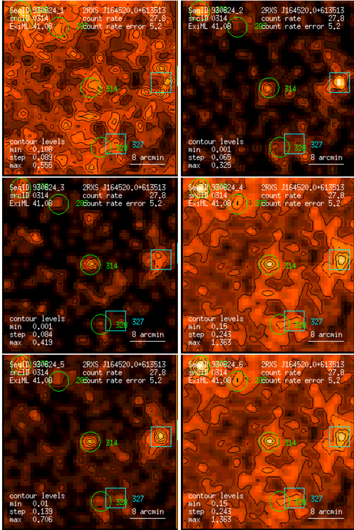
Figure 314: RASS 930624: detection 0314: band rate images, Gaussian filter: (1) PSPC channels 11 – 41, (2) 52 – 90, (3) 91 – 201, (4) 11 – 235, (5) 52 – 201, (6) 11 – 201. Broad band rates in counts/ks. Band rate contour levels in counts/ks/arcmin 2 .
