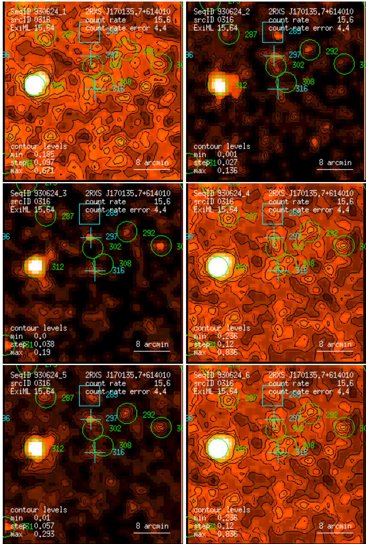
Figure 316: RASS 930624: detection 0316: band rate images, Gaussian filter: (1) PSPC channels 11 – 41, (2) 52 – 90, (3) 91 – 201, (4) 11 – 235, (5) 52 – 201, (6) 11 – 201. Broad band rates in counts/ks. Band rate contour levels in counts/ks/arcmin 2 .
