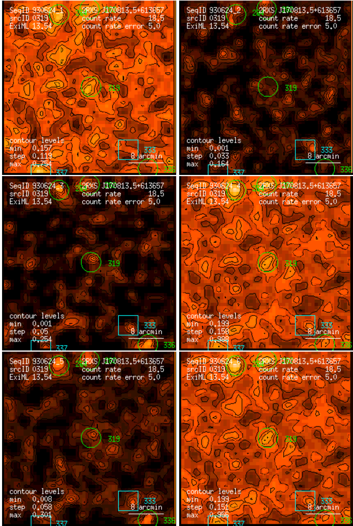
Figure 319: RASS 930624: detection 0319: band rate images, Gaussian filter: (1) PSPC channels 11 – 41, (2) 52 – 90, (3) 91 – 201, (4) 11 – 235, (5) 52 – 201, (6) 11 – 201. Broad band rates in counts/ks. Band rate contour levels in counts/ks/arcmin 2 .
