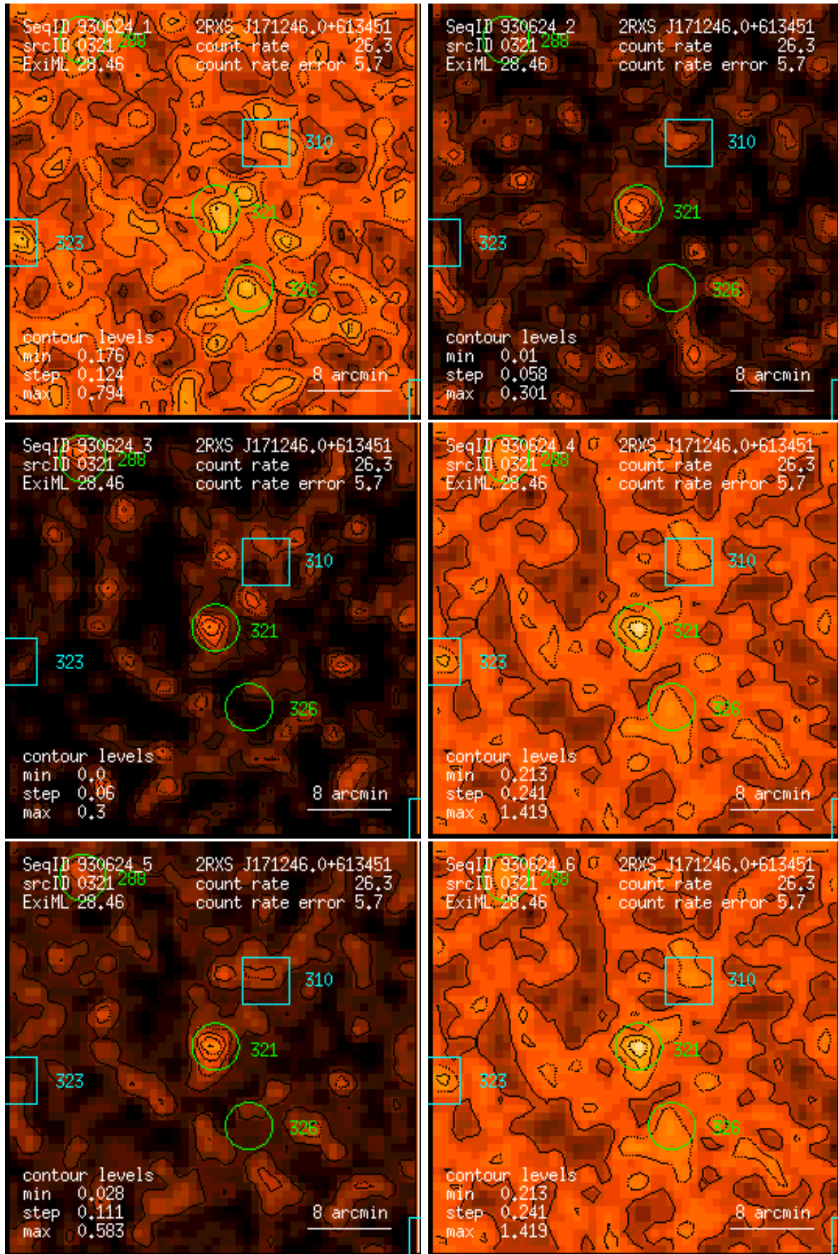
Figure 321: RASS 930624: detection 0321: band rate images, Gaussian filter: (1) PSPC channels 11 – 41, (2) 52 – 90, (3) 91 – 201, (4) 11 – 235, (5) 52 – 201, (6) 11 – 201. Broad band rates in counts/ks. Band rate contour levels in counts/ks/arcmin 2 .
