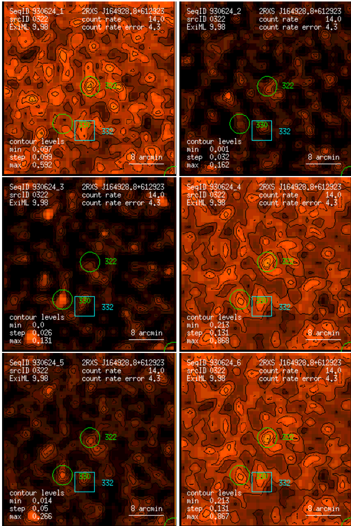
Figure 322: RASS 930624: detection 0322: band rate images, Gaussian filter: (1) PSPC channels 11 – 41, (2) 52 – 90, (3) 91 – 201, (4) 11 – 235, (5) 52 – 201, (6) 11 – 201. Broad band rates in counts/ks. Band rate contour levels in counts/ks/arcmin 2 .
