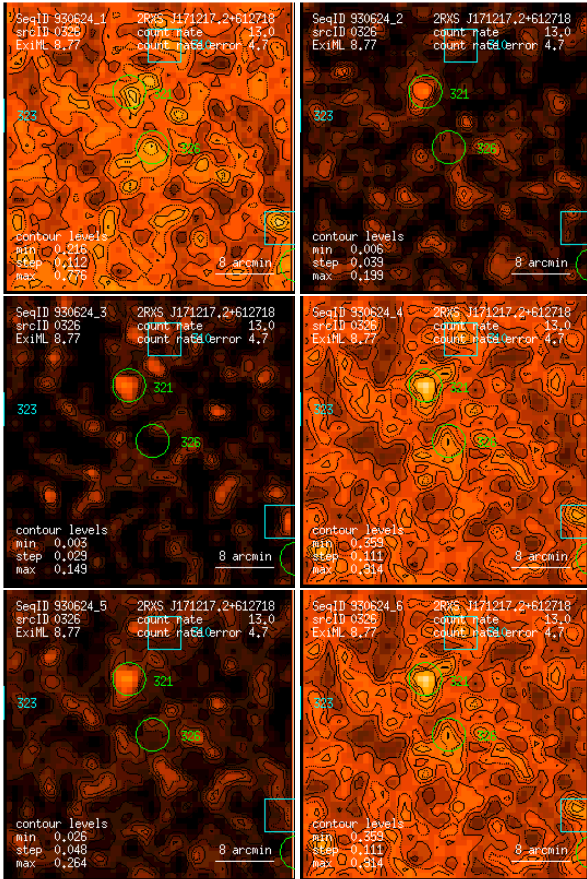
Figure 326: RASS 930624: detection 0326: band rate images, Gaussian filter: (1) PSPC channels 11 – 41, (2) 52 – 90, (3) 91 – 201, (4) 11 – 235, (5) 52 – 201, (6) 11 – 201. Broad band rates in counts/ks. Band rate contour levels in counts/ks/arcmin 2 .
