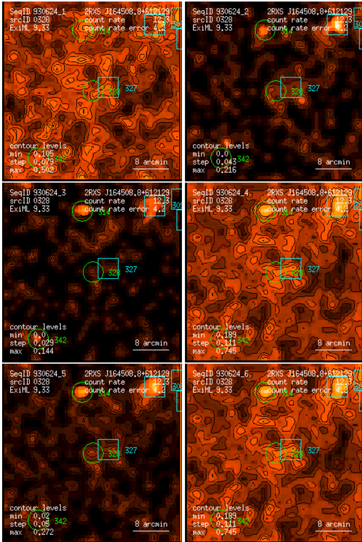
Figure 328: RASS 930624: detection 0328: band rate images, Gaussian filter: (1) PSPC channels 11 – 41, (2) 52 – 90, (3) 91 – 201, (4) 11 – 235, (5) 52 – 201, (6) 11 – 201. Broad band rates in counts/ks. Band rate contour levels in counts/ks/arcmin 2 .
