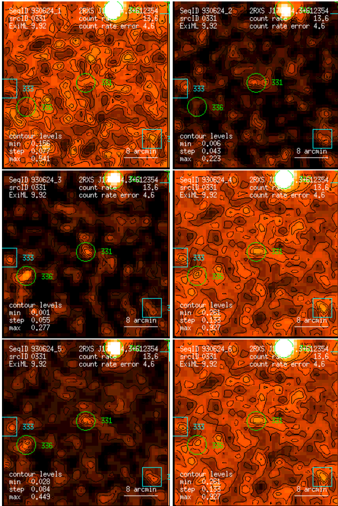
Figure 331: RASS 930624: detection 0331: band rate images, Gaussian filter: (1) PSPC channels 11 – 41, (2) 52 – 90, (3) 91 – 201, (4) 11 – 235, (5) 52 – 201, (6) 11 – 201. Broad band rates in counts/ks. Band rate contour levels in counts/ks/arcmin 2 .
