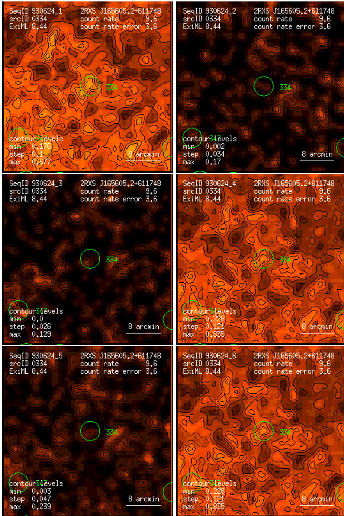
Figure 334: RASS 930624: detection 0334: band rate images, Gaussian filter: (1) PSPC channels 11 – 41, (2) 52 – 90, (3) 91 – 201, (4) 11 – 235, (5) 52 – 201, (6) 11 – 201. Broad band rates in counts/ks. Band rate contour levels in counts/ks/arcmin 2 .
