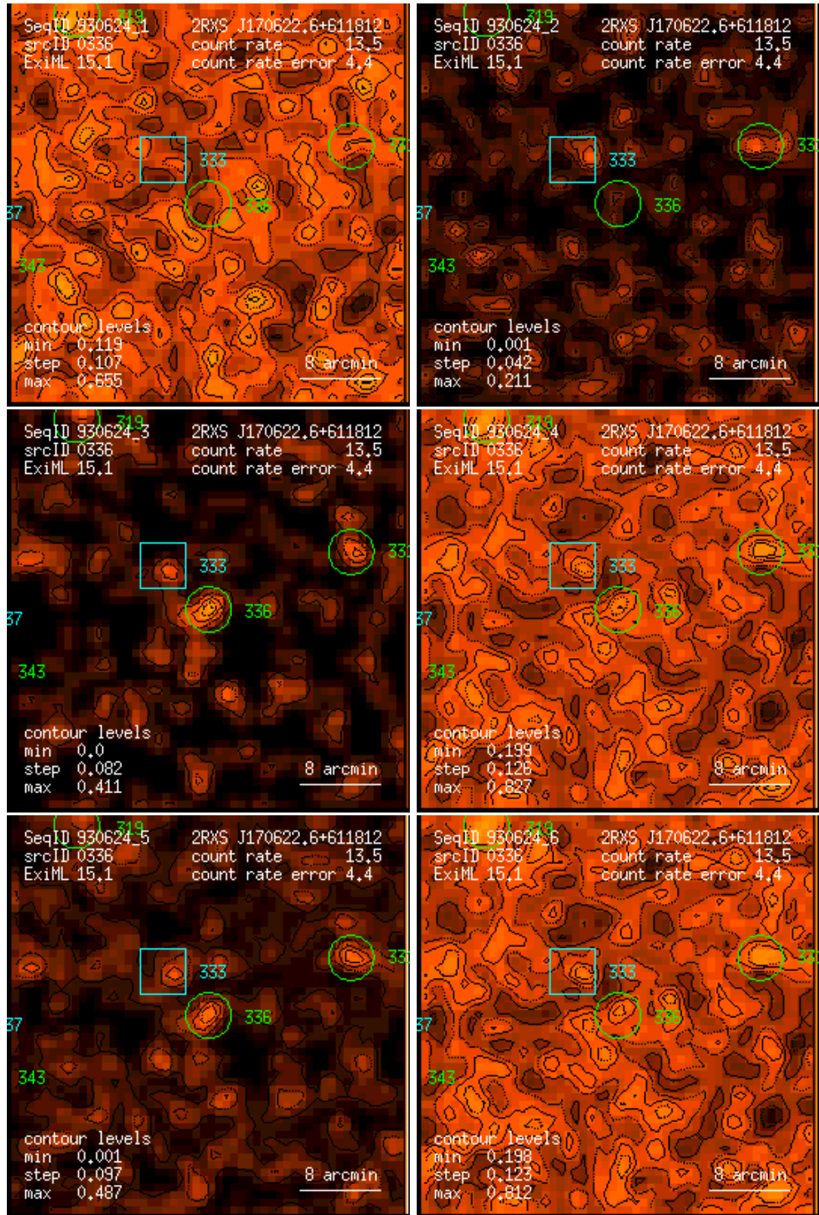
Figure 336: RASS 930624: detection 0336: band rate images, Gaussian filter: (1) PSPC channels 11 – 41, (2) 52 – 90, (3) 91 – 201, (4) 11 – 235, (5) 52 – 201, (6) 11 – 201. Broad band rates in counts/ks. Band rate contour levels in counts/ks/arcmin 2 .
