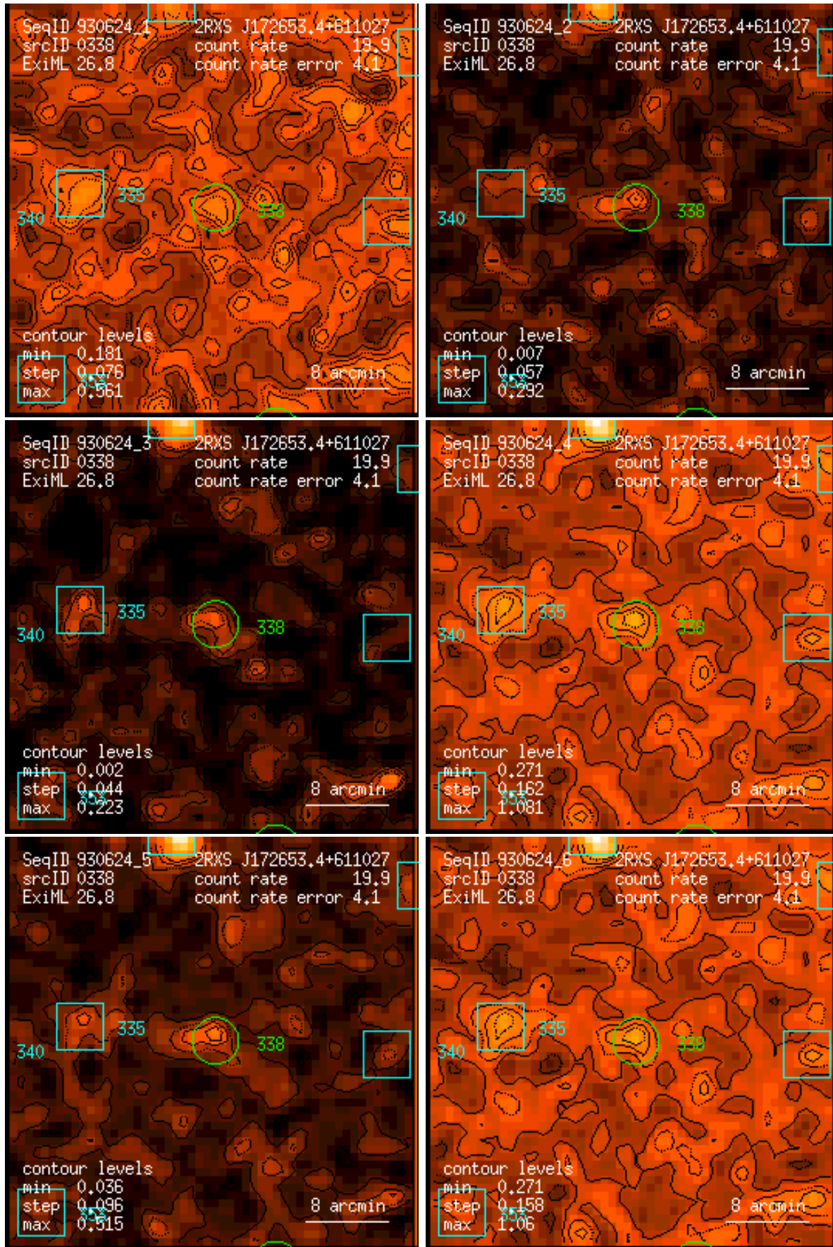
Figure 338: RASS 930624: detection 0338: band rate images, Gaussian filter: (1) PSPC channels 11 – 41, (2) 52 – 90, (3) 91 – 201, (4) 11 – 235, (5) 52 – 201, (6) 11 – 201. Broad band rates in counts/ks. Band rate contour levels in counts/ks/arcmin 2 .
