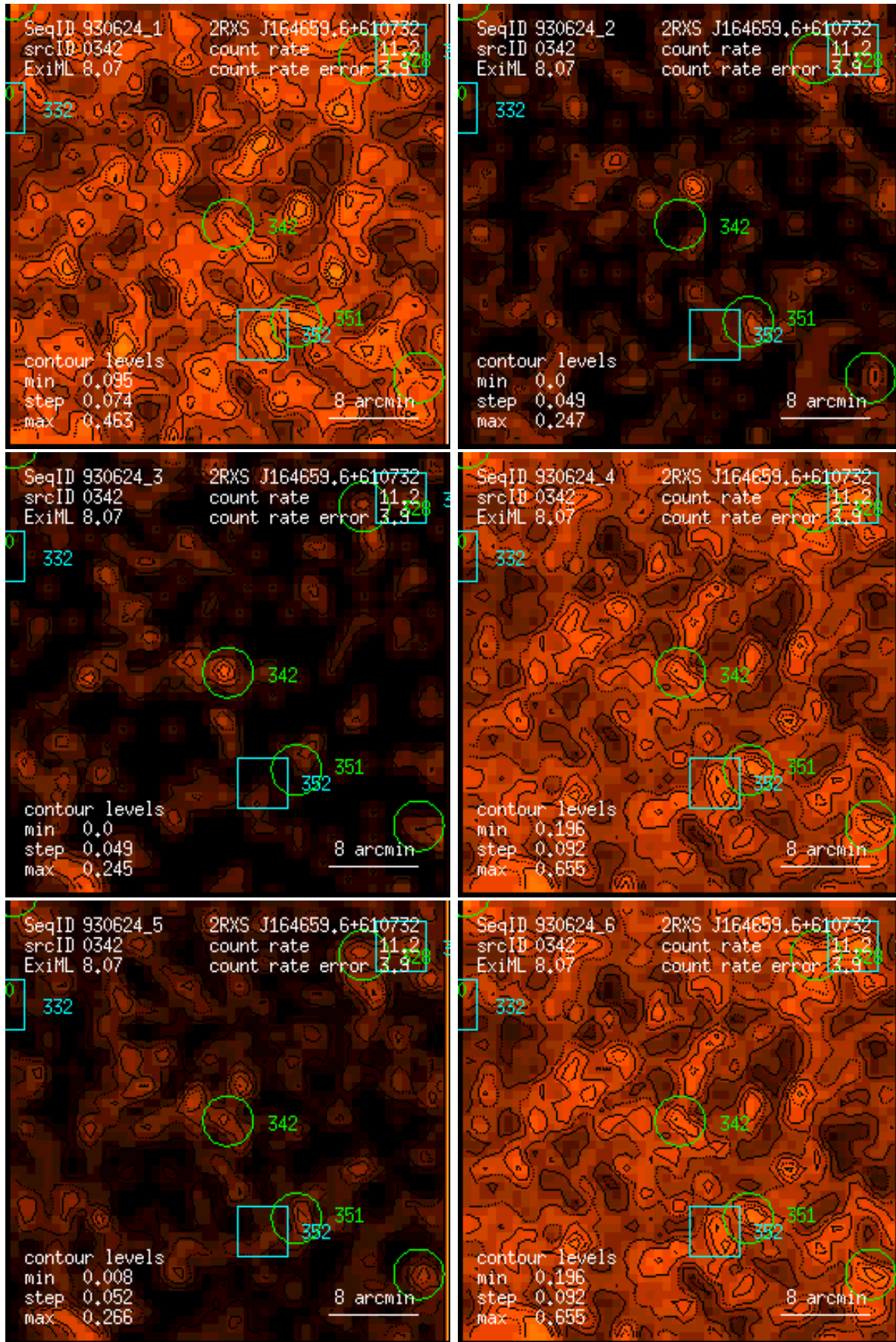
Figure 342: RASS 930624: detection 0342: band rate images, Gaussian filter: (1) PSPC channels 11 – 41, (2) 52 – 90, (3) 91 – 201, (4) 11 – 235, (5) 52 – 201, (6) 11 – 201. Broad band rates in counts/ks. Band rate contour levels in counts/ks/arcmin 2 .
