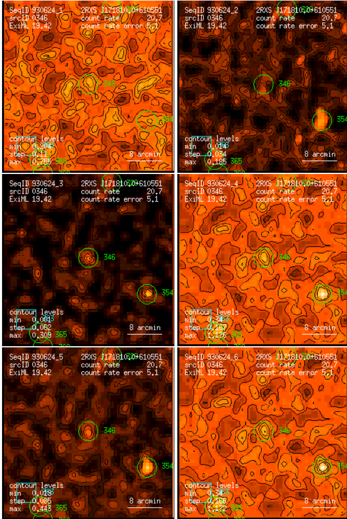
Figure 346: RASS 930624: detection 0346: band rate images, Gaussian filter: (1) PSPC channels 11 – 41, (2) 52 – 90, (3) 91 – 201, (4) 11 – 235, (5) 52 – 201, (6) 11 – 201. Broad band rates in counts/ks. Band rate contour levels in counts/ks/arcmin 2 .
