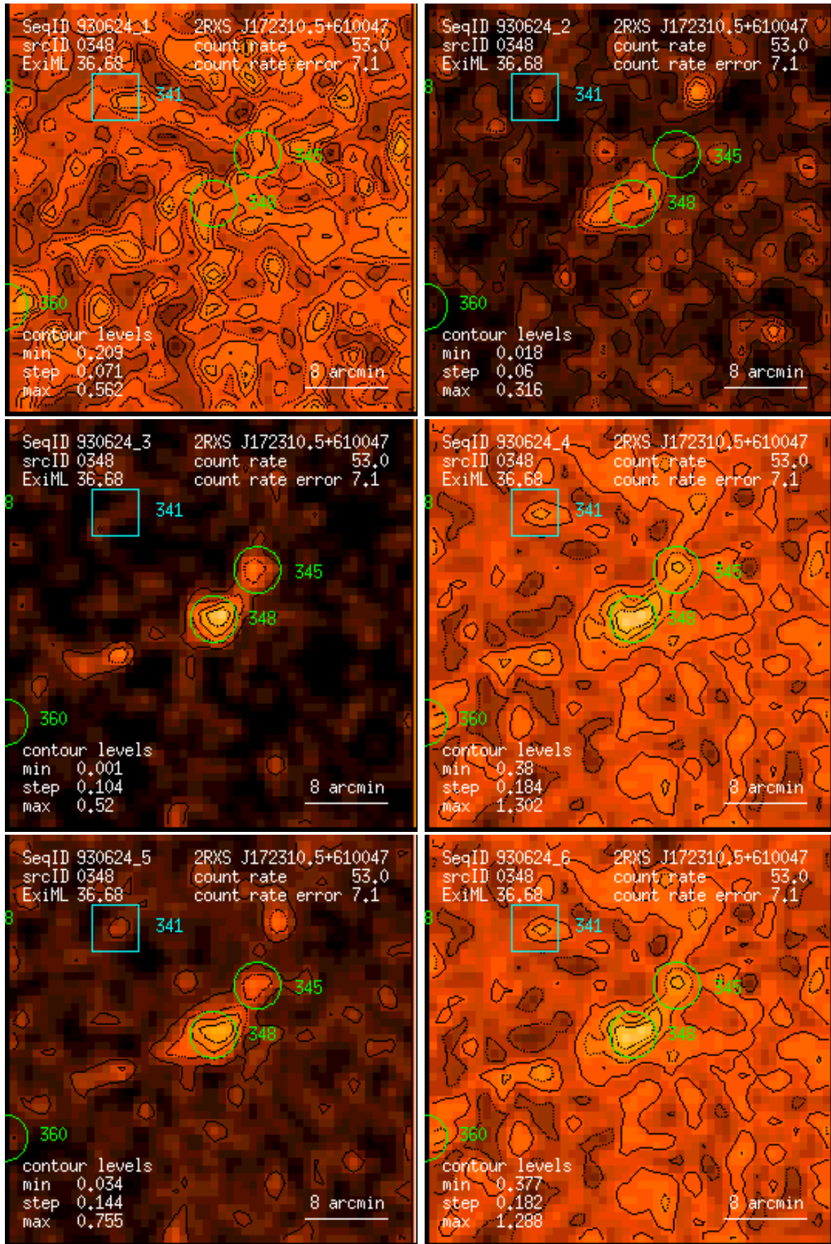
Figure 348: RASS 930624: detection 0348: band rate images, Gaussian filter: (1) PSPC channels 11 – 41, (2) 52 – 90, (3) 91 – 201, (4) 11 – 235, (5) 52 – 201, (6) 11 – 201. Broad band rates in counts/ks. Band rate contour levels in counts/ks/arcmin 2 .
