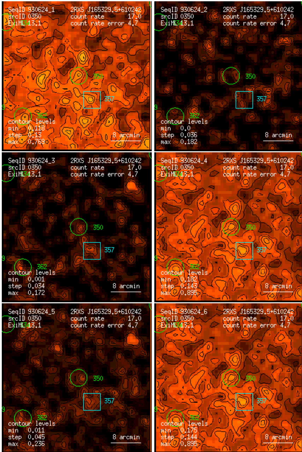
Figure 350: RASS 930624: detection 0350: band rate images, Gaussian filter: (1) PSPC channels 11 – 41, (2) 52 – 90, (3) 91 – 201, (4) 11 – 235, (5) 52 – 201, (6) 11 – 201. Broad band rates in counts/ks. Band rate contour levels in counts/ks/arcmin 2 .
