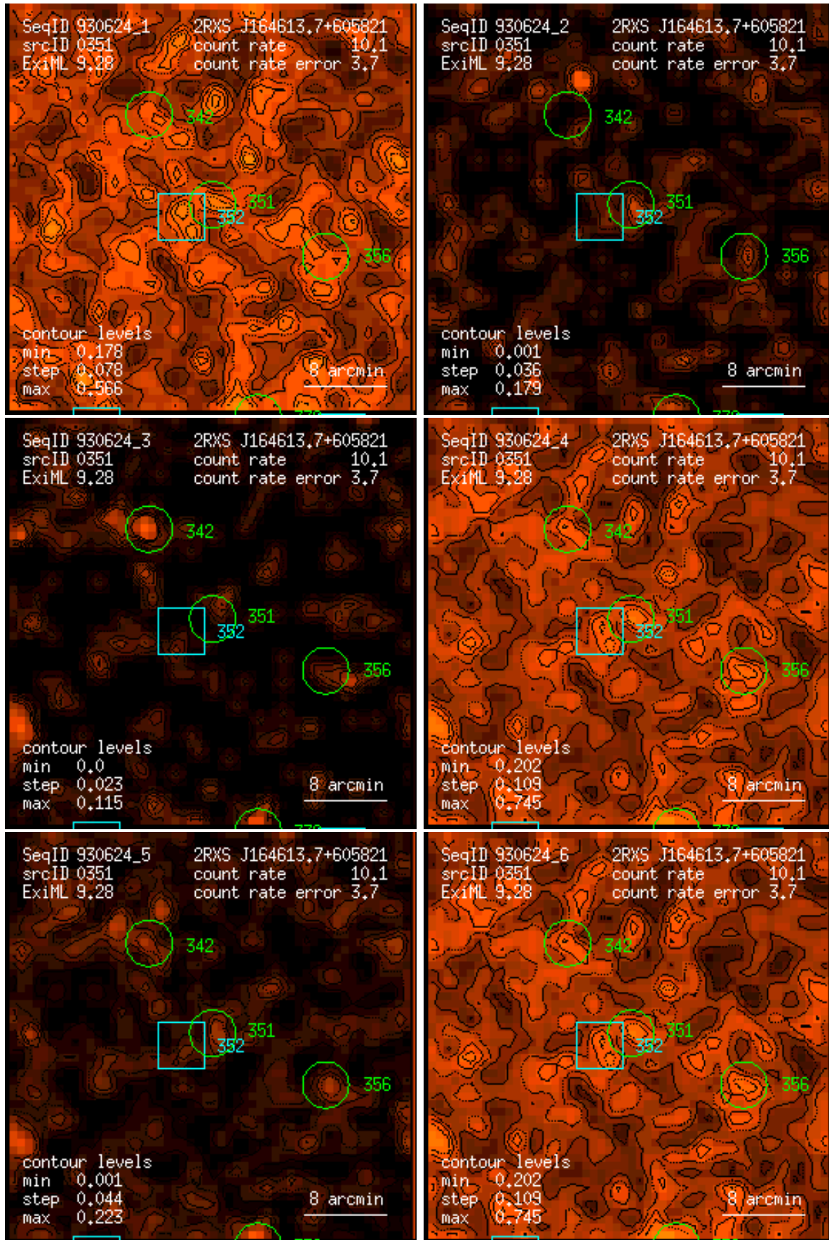
Figure 351: RASS 930624: detection 0351: band rate images, Gaussian filter: (1) PSPC channels 11 – 41, (2) 52 – 90, (3) 91 – 201, (4) 11 – 235, (5) 52 – 201, (6) 11 – 201. Broad band rates in counts/ks. Band rate contour levels in counts/ks/arcmin 2 .
