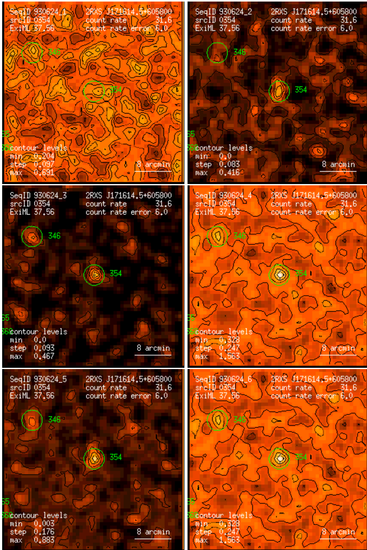
Figure 354: RASS 930624: detection 0354: band rate images, Gaussian filter: (1) PSPC channels 11 – 41, (2) 52 – 90, (3) 91 – 201, (4) 11 – 235, (5) 52 – 201, (6) 11 – 201. Broad band rates in counts/ks. Band rate contour levels in counts/ks/arcmin 2 .
