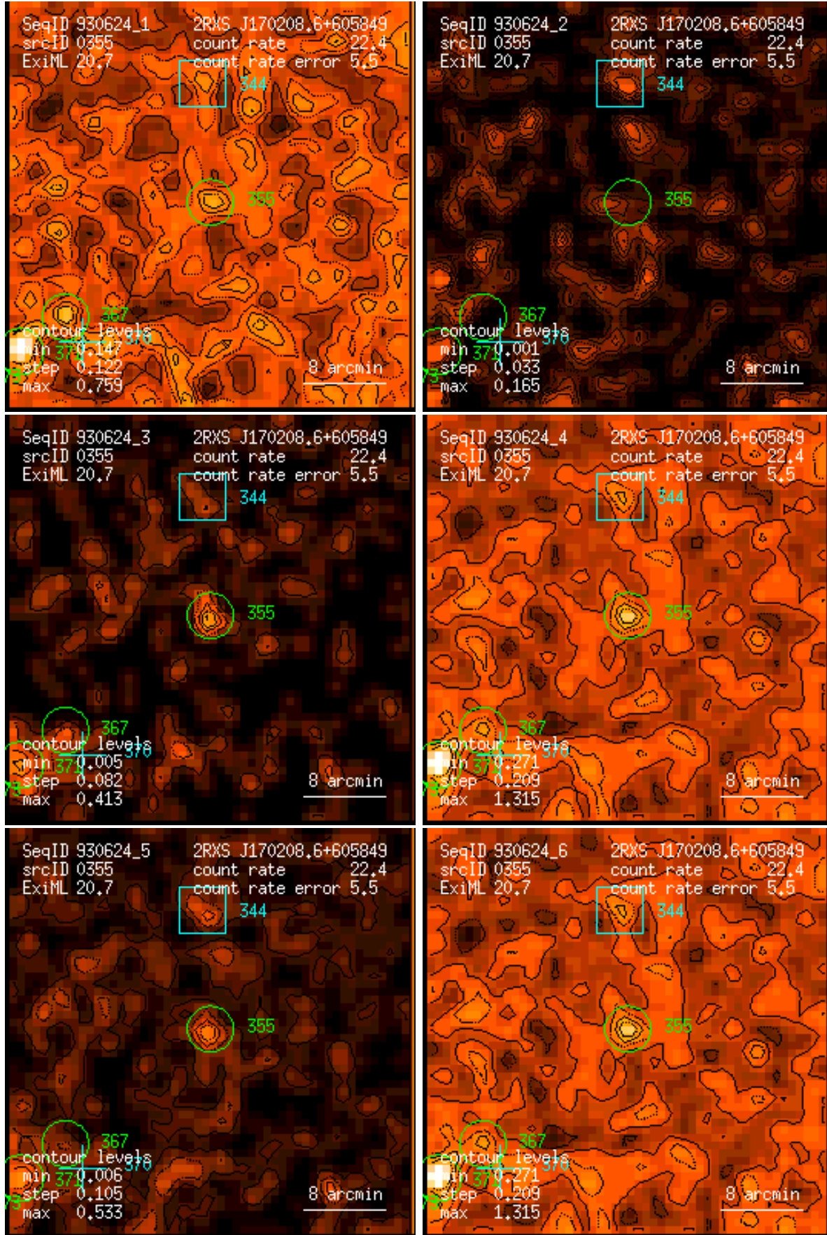
Figure 355: RASS 930624: detection 0355: band rate images, Gaussian filter: (1) PSPC channels 11 – 41, (2) 52 – 90, (3) 91 – 201, (4) 11 – 235, (5) 52 – 201, (6) 11 – 201. Broad band rates in counts/ks. Band rate contour levels in counts/ks/arcmin 2 .
