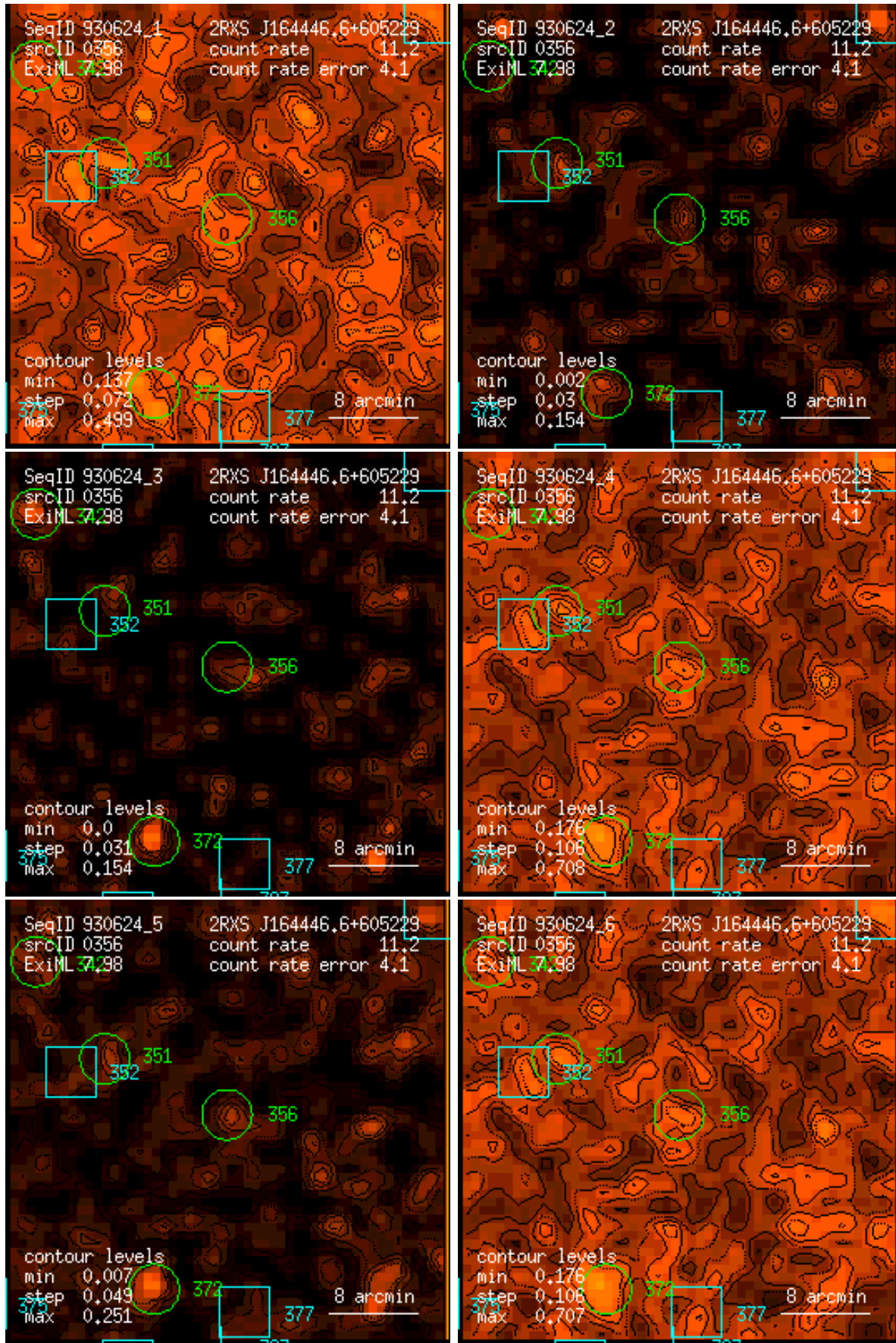
Figure 356: RASS 930624: detection 0356: band rate images, Gaussian filter: (1) PSPC channels 11 – 41, (2) 52 – 90, (3) 91 – 201, (4) 11 – 235, (5) 52 – 201, (6) 11 – 201. Broad band rates in counts/ks. Band rate contour levels in counts/ks/arcmin 2 .
