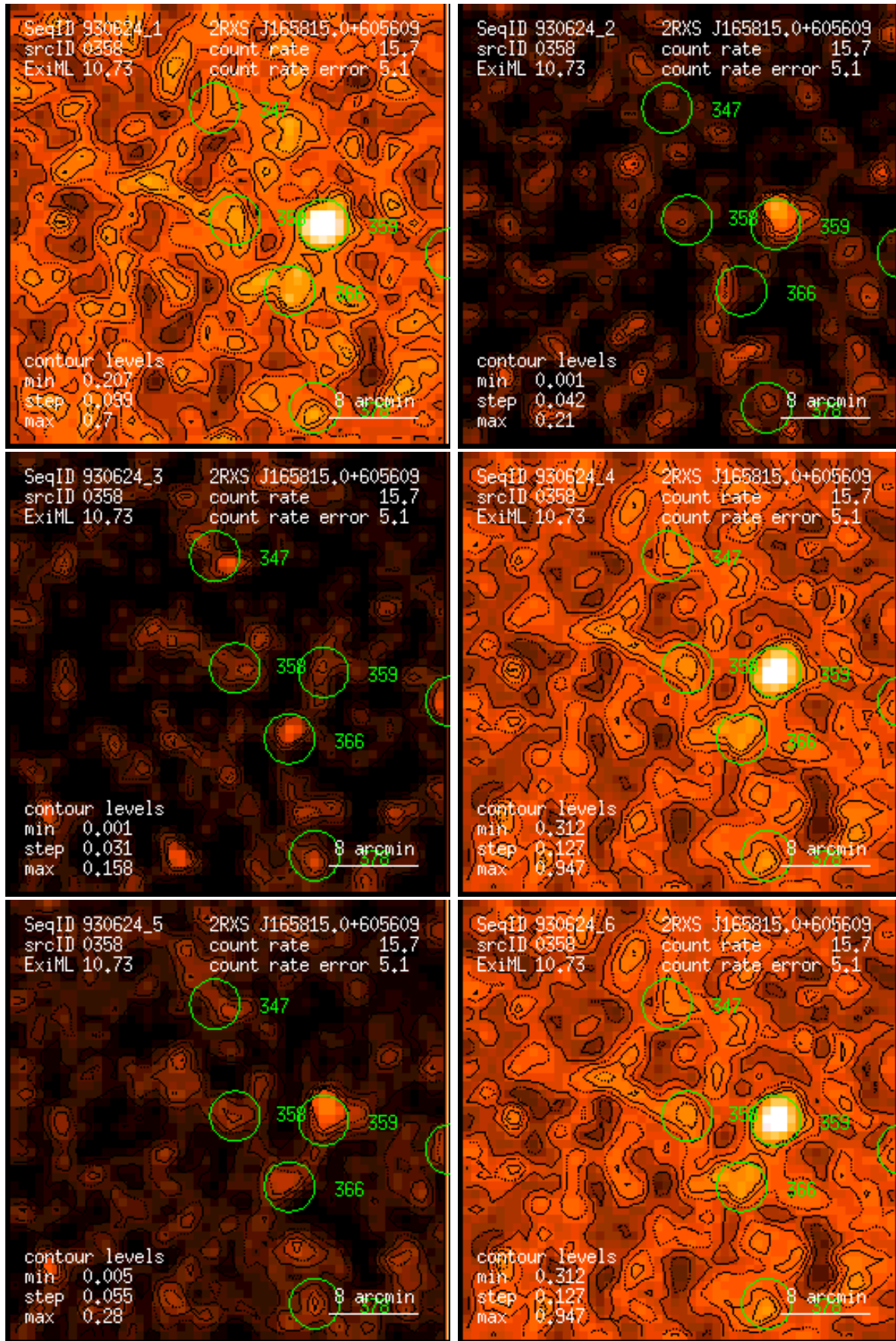
Figure 358: RASS 930624: detection 0358: band rate images, Gaussian filter: (1) PSPC channels 11 – 41, (2) 52 – 90, (3) 91 – 201, (4) 11 – 235, (5) 52 – 201, (6) 11 – 201. Broad band rates in counts/ks. Band rate contour levels in counts/ks/arcmin 2 .
