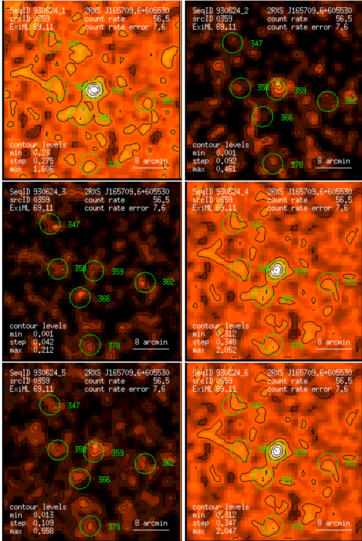
Figure 359: RASS 930624: detection 0359: band rate images, Gaussian filter: (1) PSPC channels 11 – 41, (2) 52 – 90, (3) 91 – 201, (4) 11 – 235, (5) 52 – 201, (6) 11 – 201. Broad band rates in counts/ks. Band rate contour levels in counts/ks/arcmin 2 .
