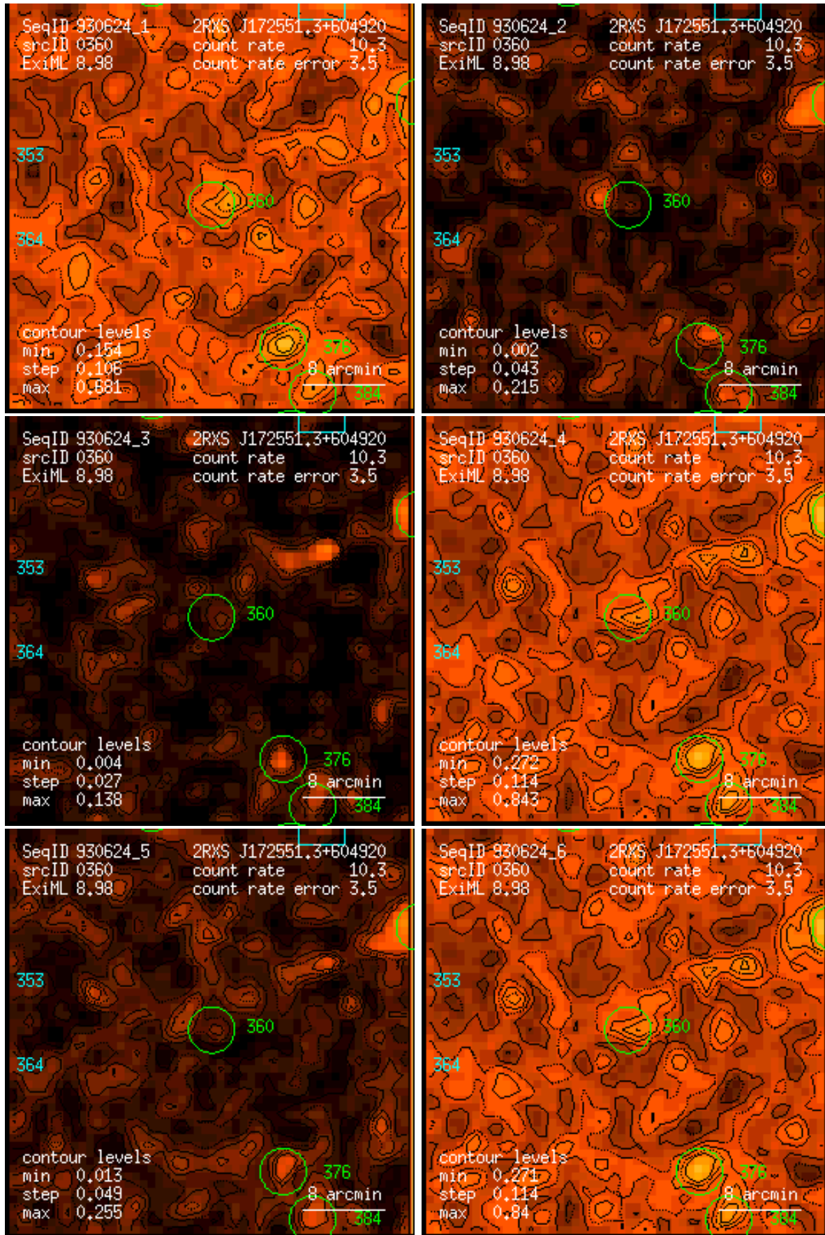
Figure 360: RASS 930624: detection 0360: band rate images, Gaussian filter: (1) PSPC channels 11 – 41, (2) 52 – 90, (3) 91 – 201, (4) 11 – 235, (5) 52 – 201, (6) 11 – 201. Broad band rates in counts/ks. Band rate contour levels in counts/ks/arcmin 2 .
