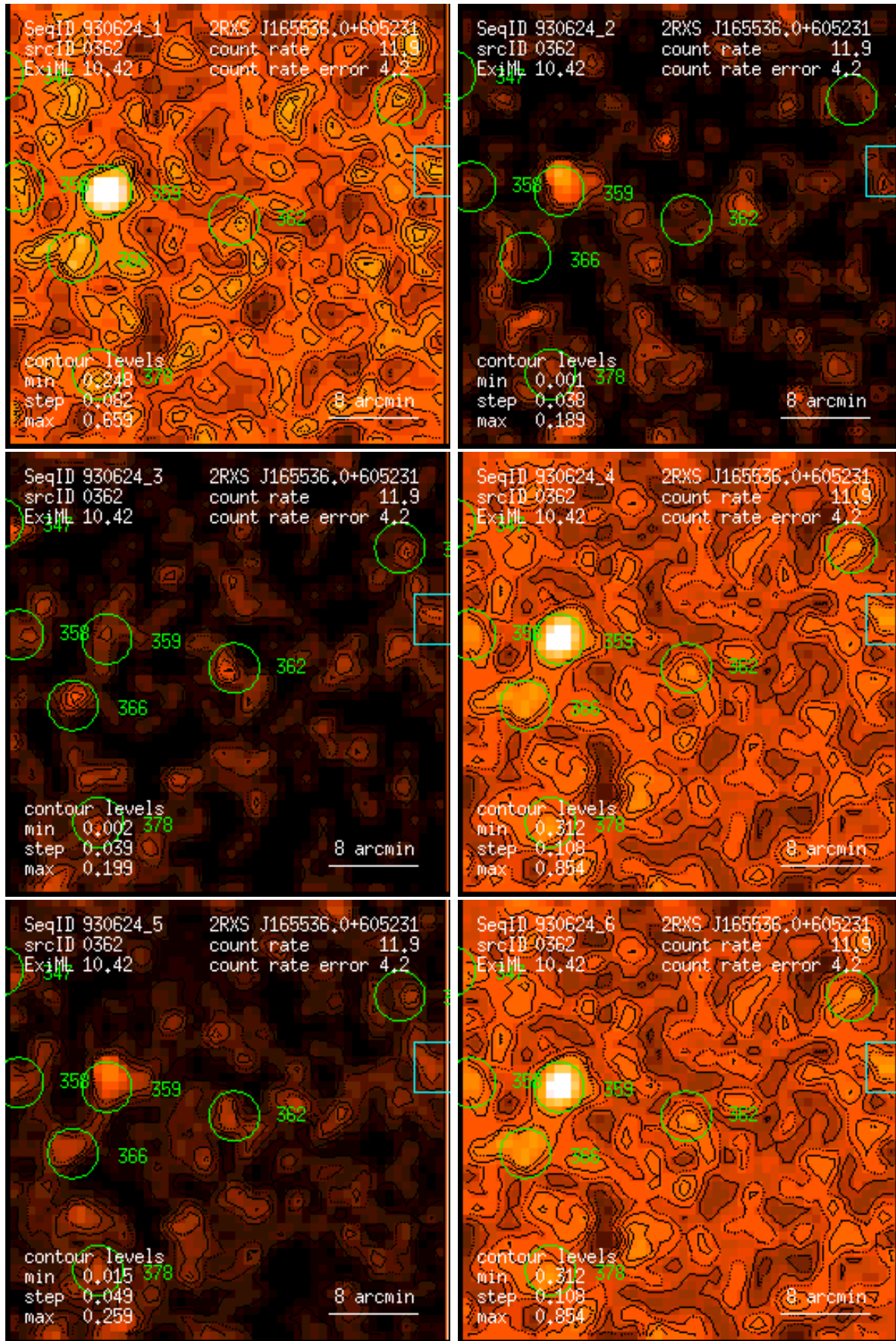
Figure 362: RASS 930624: detection 0362: band rate images, Gaussian filter: (1) PSPC channels 11 – 41, (2) 52 – 90, (3) 91 – 201, (4) 11 – 235, (5) 52 – 201, (6) 11 – 201. Broad band rates in counts/ks. Band rate contour levels in counts/ks/arcmin 2 .
