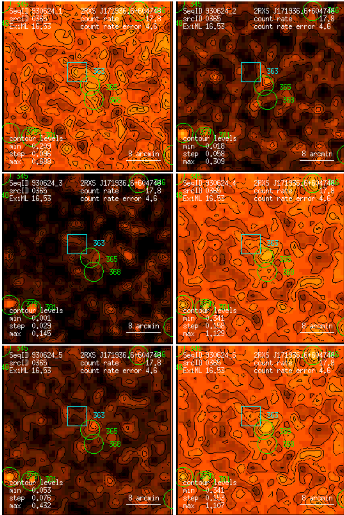
Figure 365: RASS 930624: detection 0365: band rate images, Gaussian filter: (1) PSPC channels 11 – 41, (2) 52 – 90, (3) 91 – 201, (4) 11 – 235, (5) 52 – 201, (6) 11 – 201. Broad band rates in counts/ks. Band rate contour levels in counts/ks/arcmin 2 .
