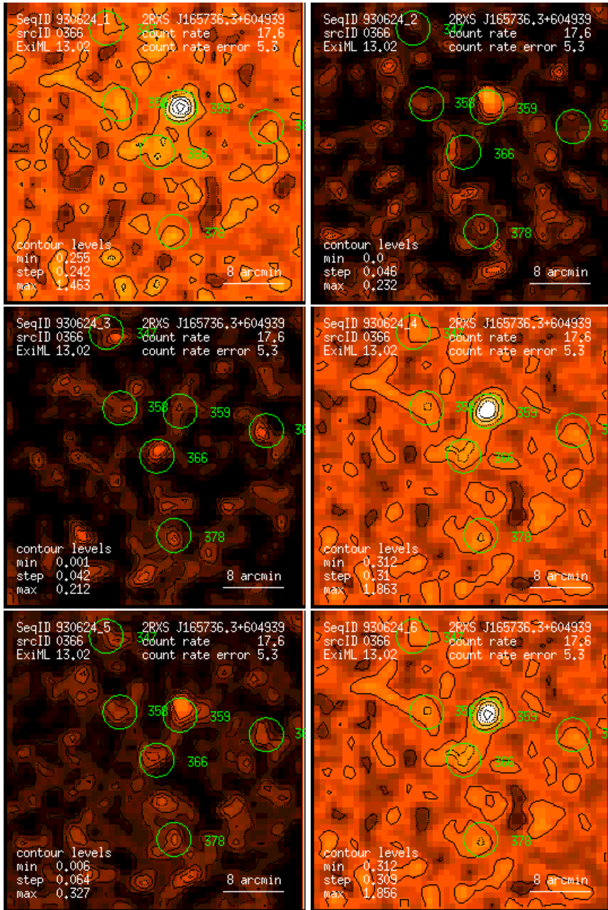
Figure 366: RASS 930624: detection 0366: band rate images, Gaussian filter: (1) PSPC channels 11 – 41, (2) 52 – 90, (3) 91 – 201, (4) 11 – 235, (5) 52 – 201, (6) 11 – 201. Broad band rates in counts/ks. Band rate contour levels in counts/ks/arcmin 2 .
