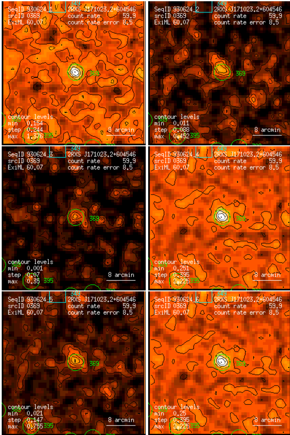
Figure 369: RASS 930624: detection 0369: band rate images, Gaussian filter: (1) PSPC channels 11 – 41, (2) 52 – 90, (3) 91 – 201, (4) 11 – 235, (5) 52 – 201, (6) 11 – 201. Broad band rates in counts/ks. Band rate contour levels in counts/ks/arcmin 2 .
