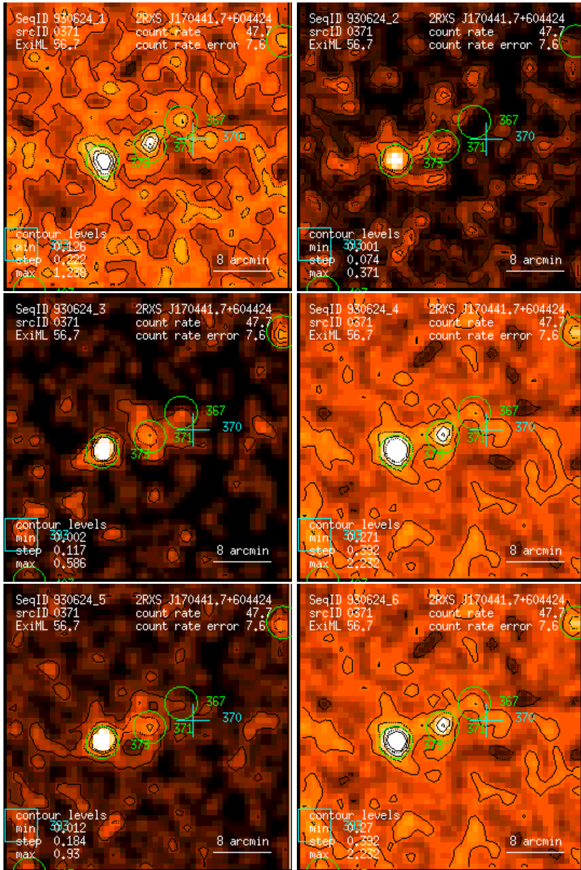
Figure 371: RASS 930624: detection 0371: band rate images, Gaussian filter: (1) PSPC channels 11 – 41, (2) 52 – 90, (3) 91 – 201, (4) 11 – 235, (5) 52 – 201, (6) 11 – 201. Broad band rates in counts/ks. Band rate contour levels in counts/ks/arcmin 2 .
