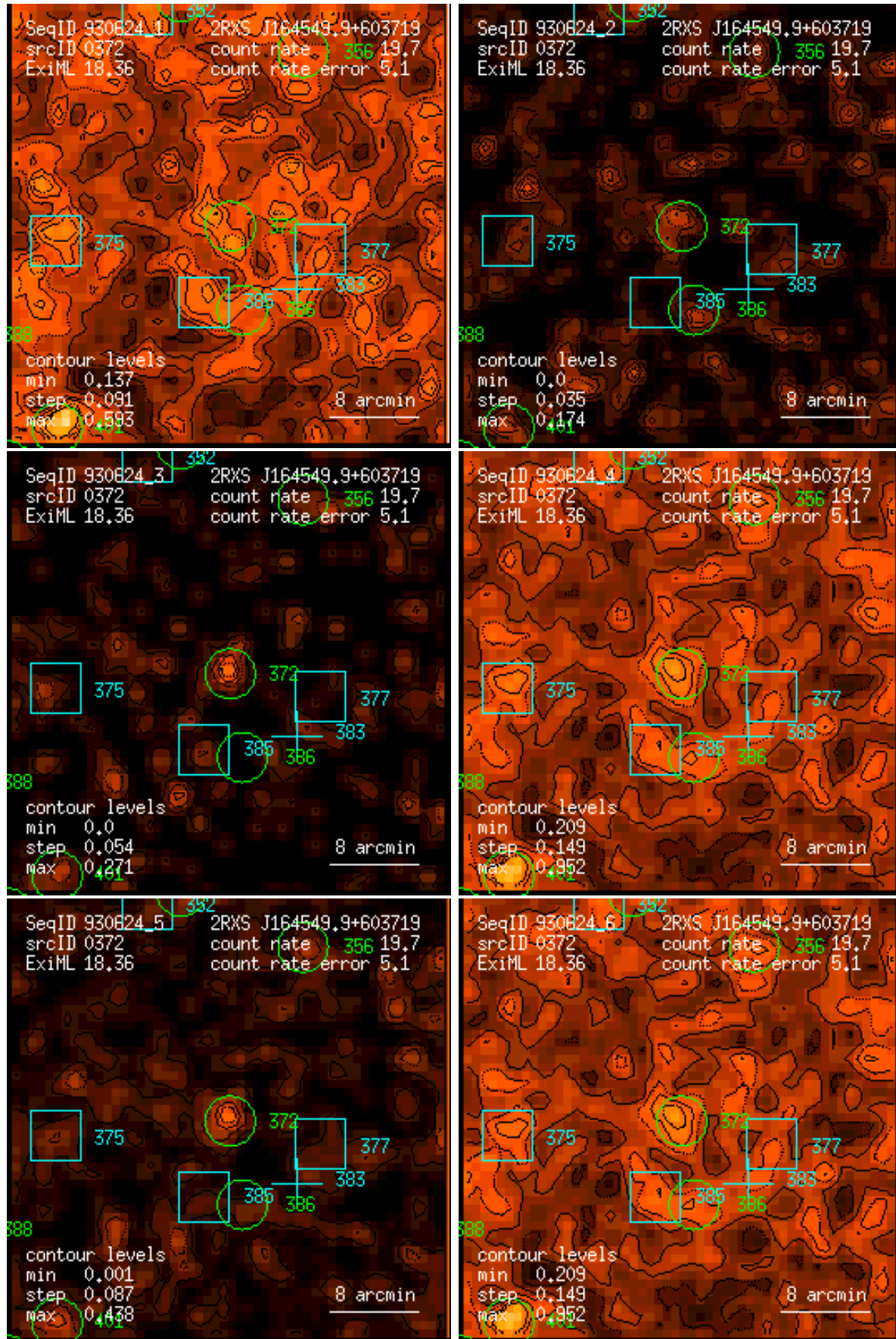
Figure 372: RASS 930624: detection 0372: band rate images, Gaussian filter: (1) PSPC channels 11 – 41, (2) 52 – 90, (3) 91 – 201, (4) 11 – 235, (5) 52 – 201, (6) 11 – 201. Broad band rates in counts/ks. Band rate contour levels in counts/ks/arcmin 2 .
