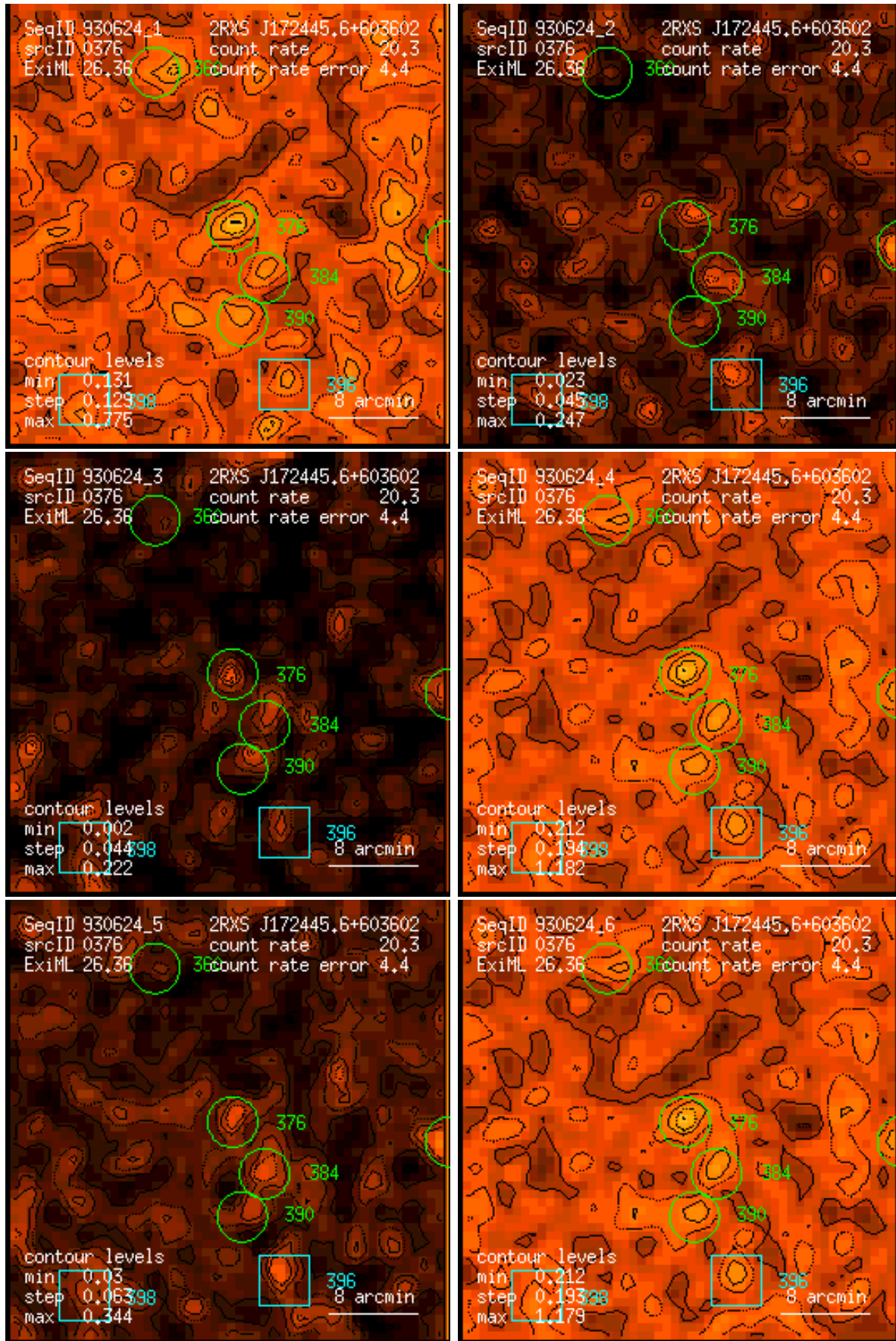
Figure 376: RASS 930624: detection 0376: band rate images, Gaussian filter: (1) PSPC channels 11 – 41, (2) 52 – 90, (3) 91 – 201, (4) 11 – 235, (5) 52 – 201, (6) 11 – 201. Broad band rates in counts/ks. Band rate contour levels in counts/ks/arcmin 2 .
