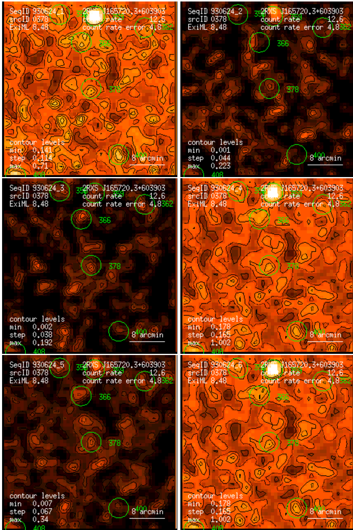
Figure 378: RASS 930624: detection 0378: band rate images, Gaussian filter: (1) PSPC channels 11 – 41, (2) 52 – 90, (3) 91 – 201, (4) 11 – 235, (5) 52 – 201, (6) 11 – 201. Broad band rates in counts/ks. Band rate contour levels in counts/ks/arcmin 2 .
