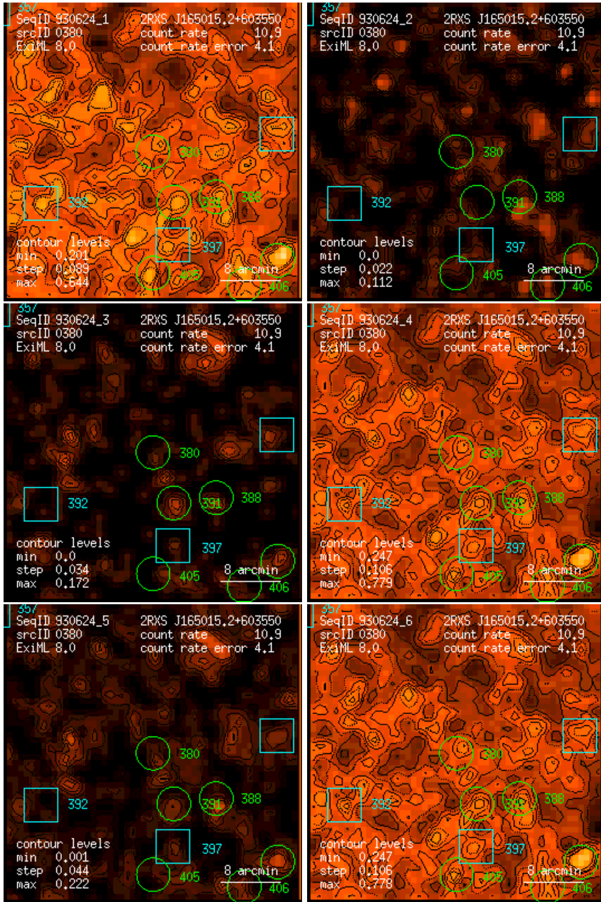
Figure 380: RASS 930624: detection 0380: band rate images, Gaussian filter: (1) PSPC channels 11 – 41, (2) 52 – 90, (3) 91 – 201, (4) 11 – 235, (5) 52 – 201, (6) 11 – 201. Broad band rates in counts/ks. Band rate contour levels in counts/ks/arcmin 2 .
