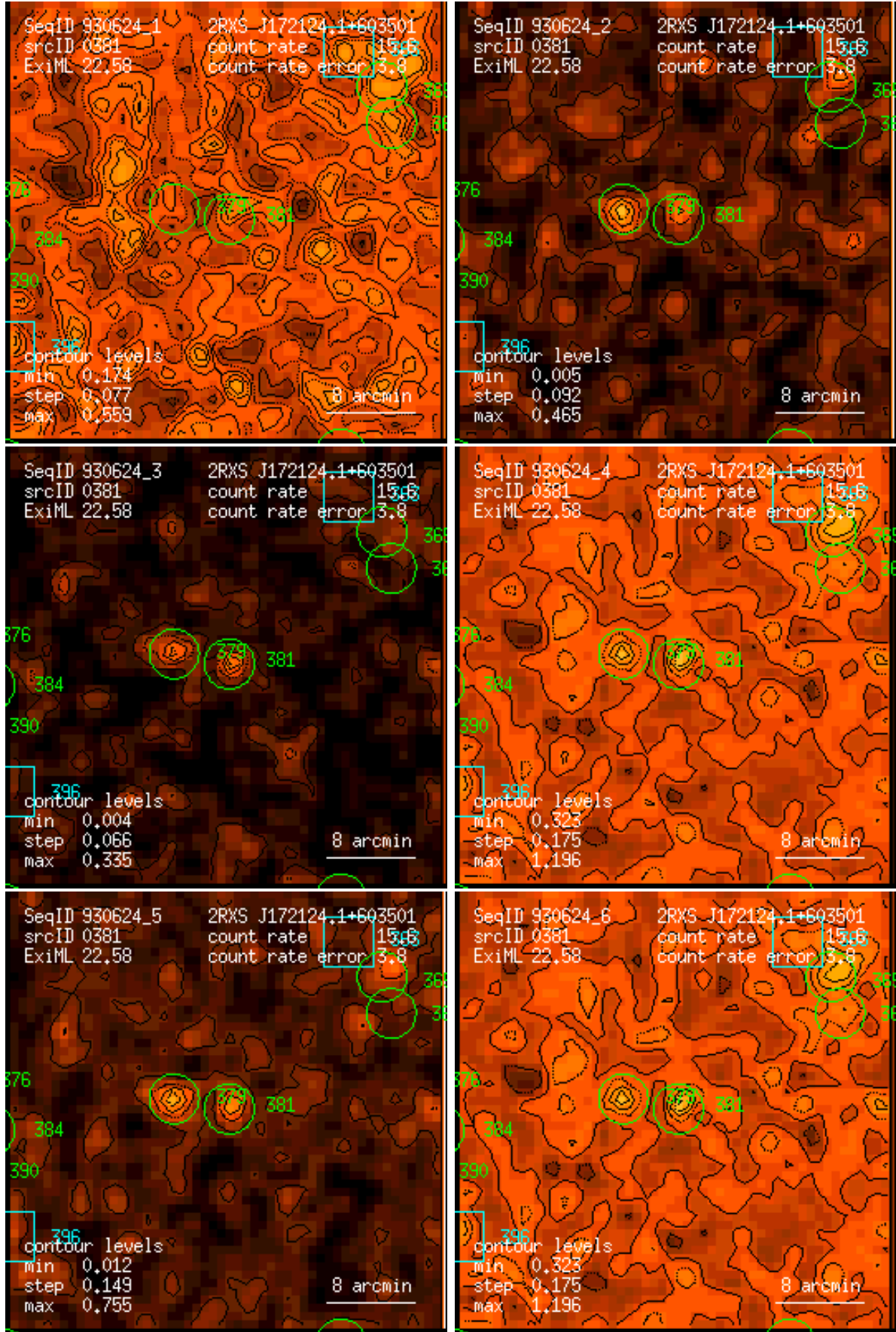
Figure 381: RASS 930624: detection 0381: band rate images, Gaussian filter: (1) PSPC channels 11 – 41, (2) 52 – 90, (3) 91 – 201, (4) 11 – 235, (5) 52 – 201, (6) 11 – 201. Broad band rates in counts/ks. Band rate contour levels in counts/ks/arcmin 2 .
