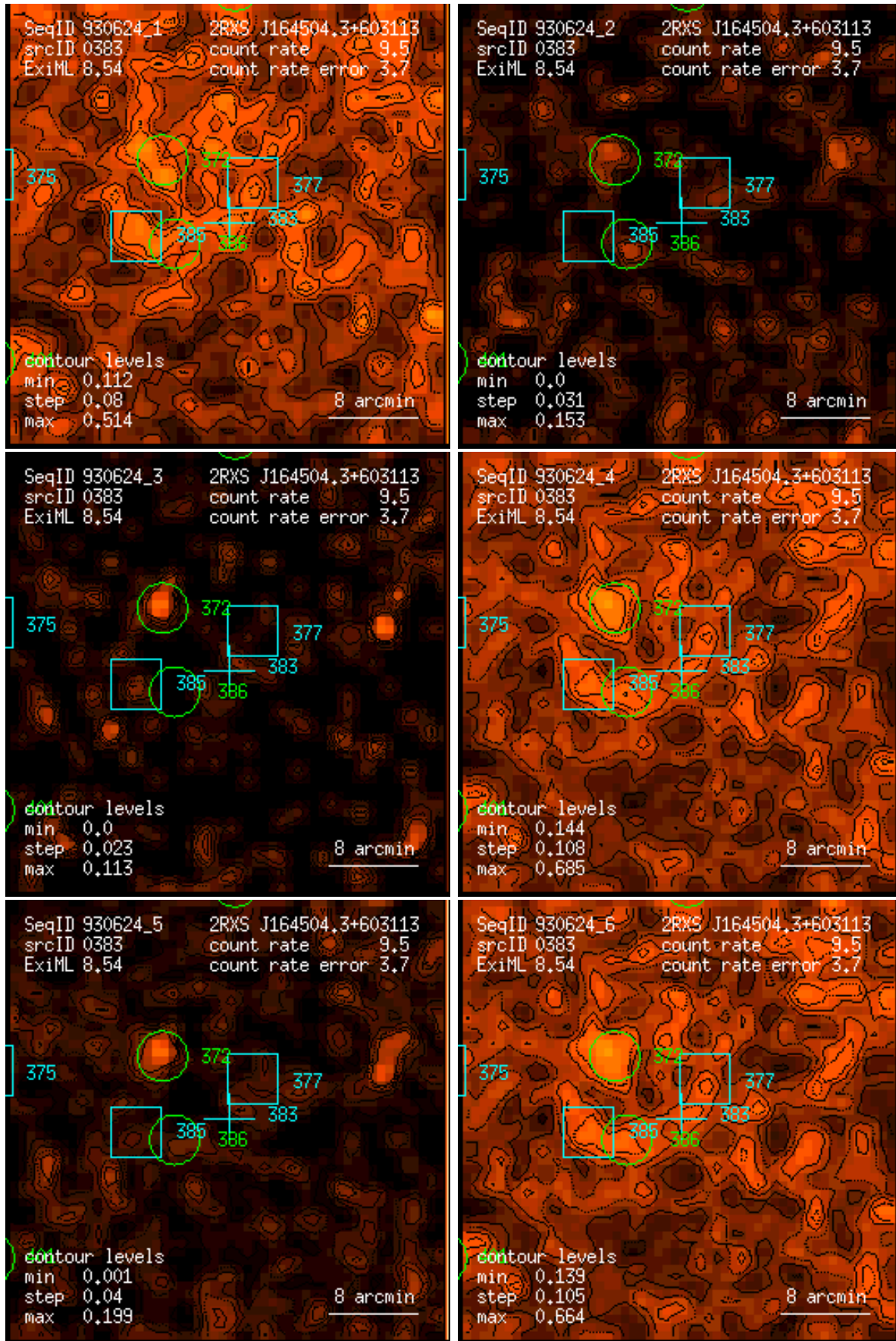
Figure 383: RASS 930624: detection 0383: band rate images, Gaussian filter: (1) PSPC channels 11 – 41, (2) 52 – 90, (3) 91 – 201, (4) 11 – 235, (5) 52 – 201, (6) 11 – 201. Broad band rates in counts/ks. Band rate contour levels in counts/ks/arcmin 2 .
