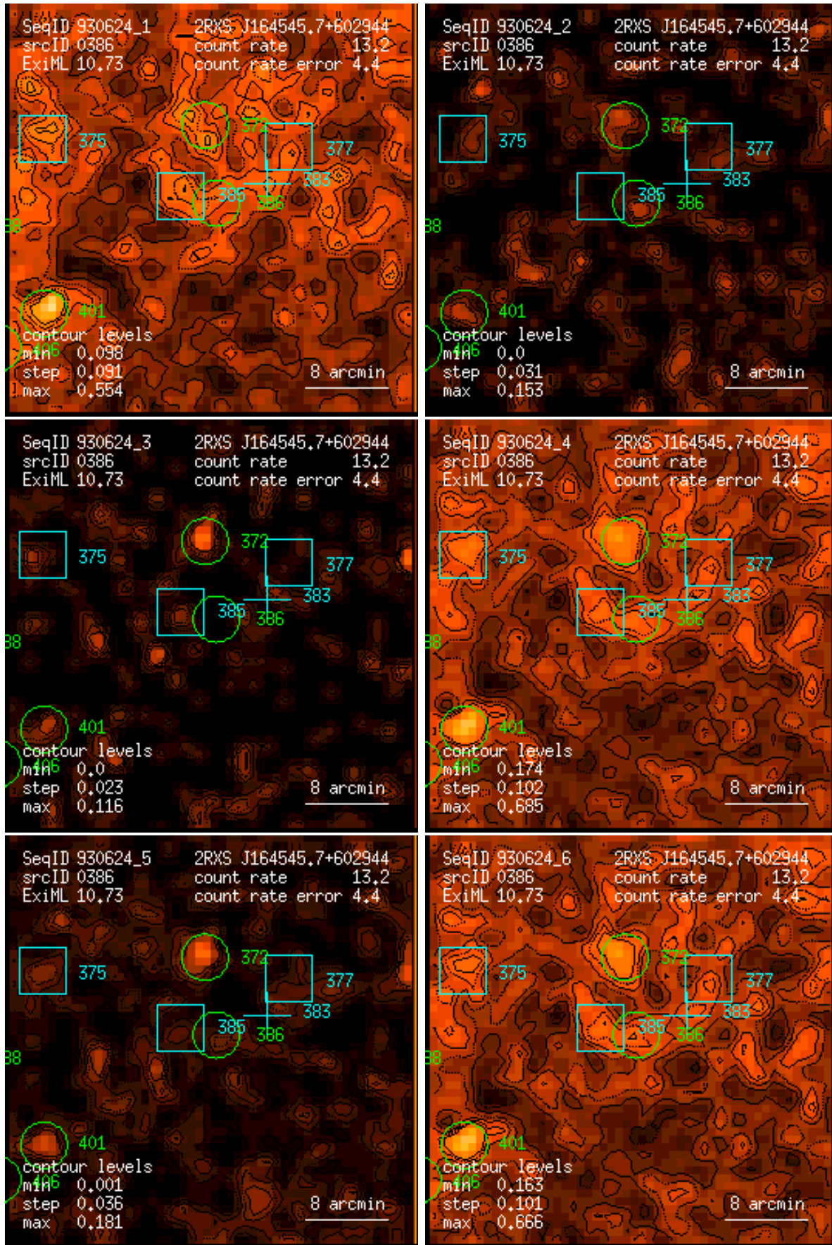
Figure 386: RASS 930624: detection 0386: band rate images, Gaussian filter: (1) PSPC channels 11 – 41, (2) 52 – 90, (3) 91 – 201, (4) 11 – 235, (5) 52 – 201, (6) 11 – 201. Broad band rates in counts/ks. Band rate contour levels in counts/ks/arcmin 2 .
