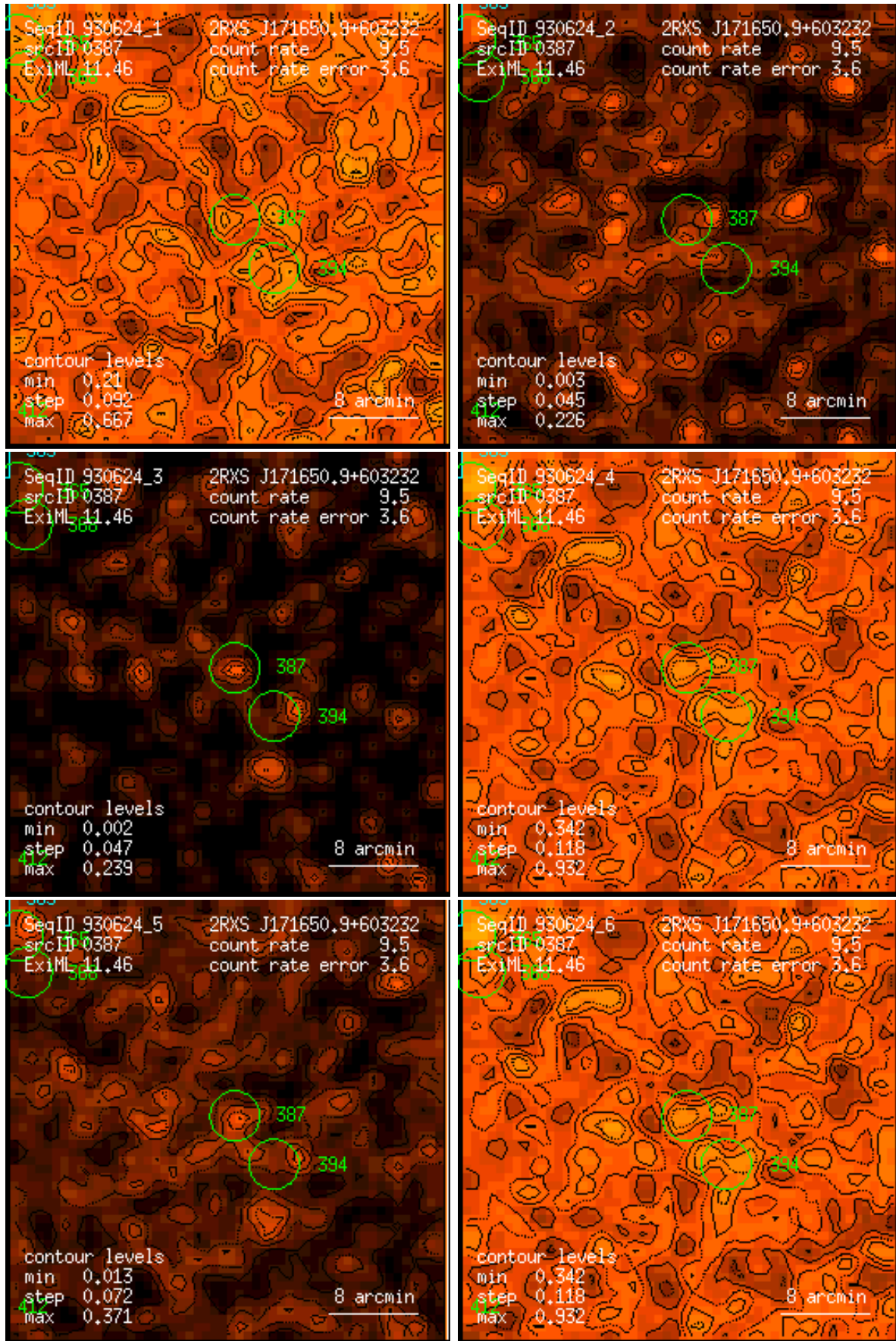
Figure 387: RASS 930624: detection 0387: band rate images, Gaussian filter: (1) PSPC channels 11 – 41, (2) 52 – 90, (3) 91 – 201, (4) 11 – 235, (5) 52 – 201, (6) 11 – 201. Broad band rates in counts/ks. Band rate contour levels in counts/ks/arcmin 2 .
