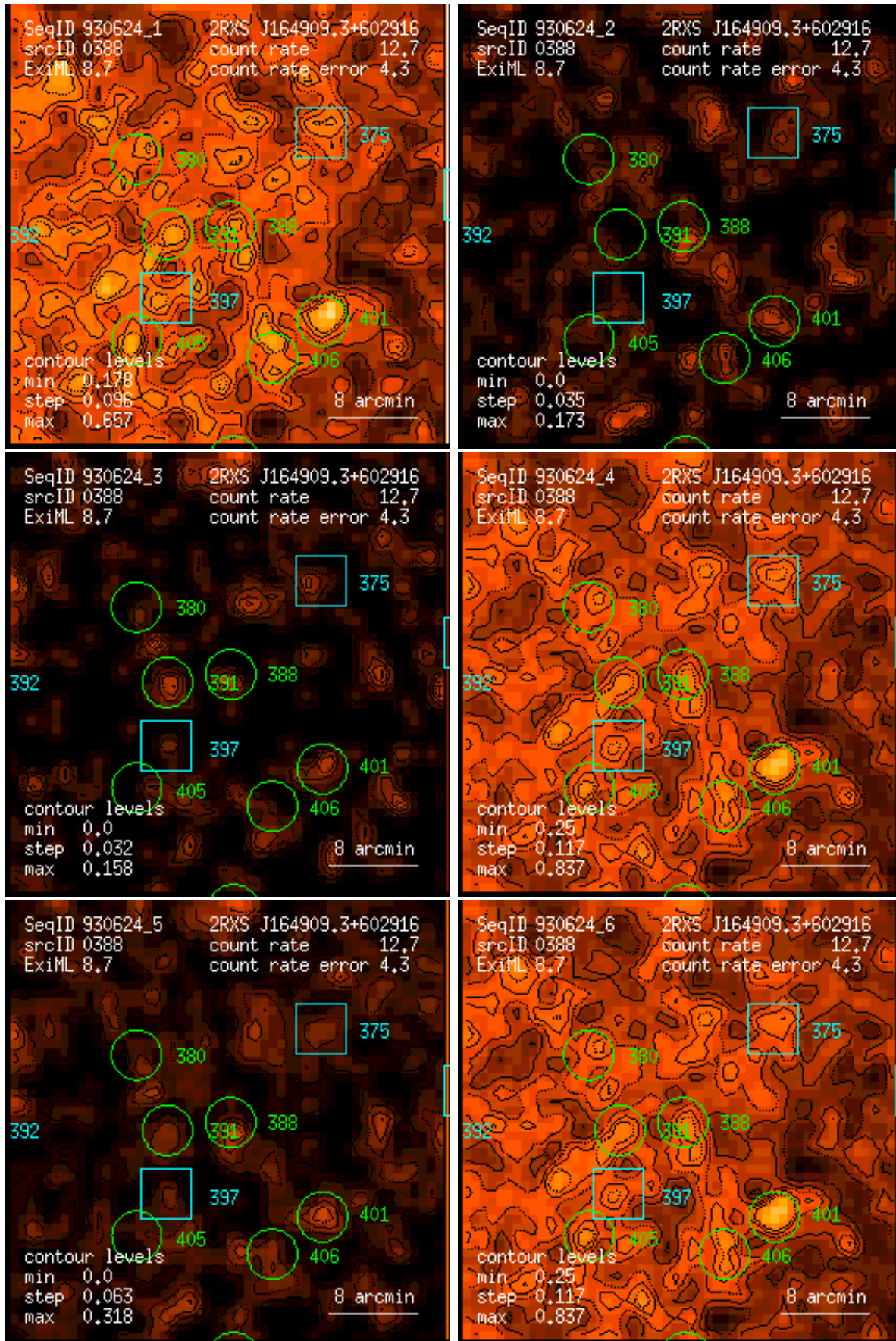
Figure 388: RASS 930624: detection 0388: band rate images, Gaussian filter: (1) PSPC channels 11 – 41, (2) 52 – 90, (3) 91 – 201, (4) 11 – 235, (5) 52 – 201, (6) 11 – 201. Broad band rates in counts/ks. Band rate contour levels in counts/ks/arcmin 2 .
