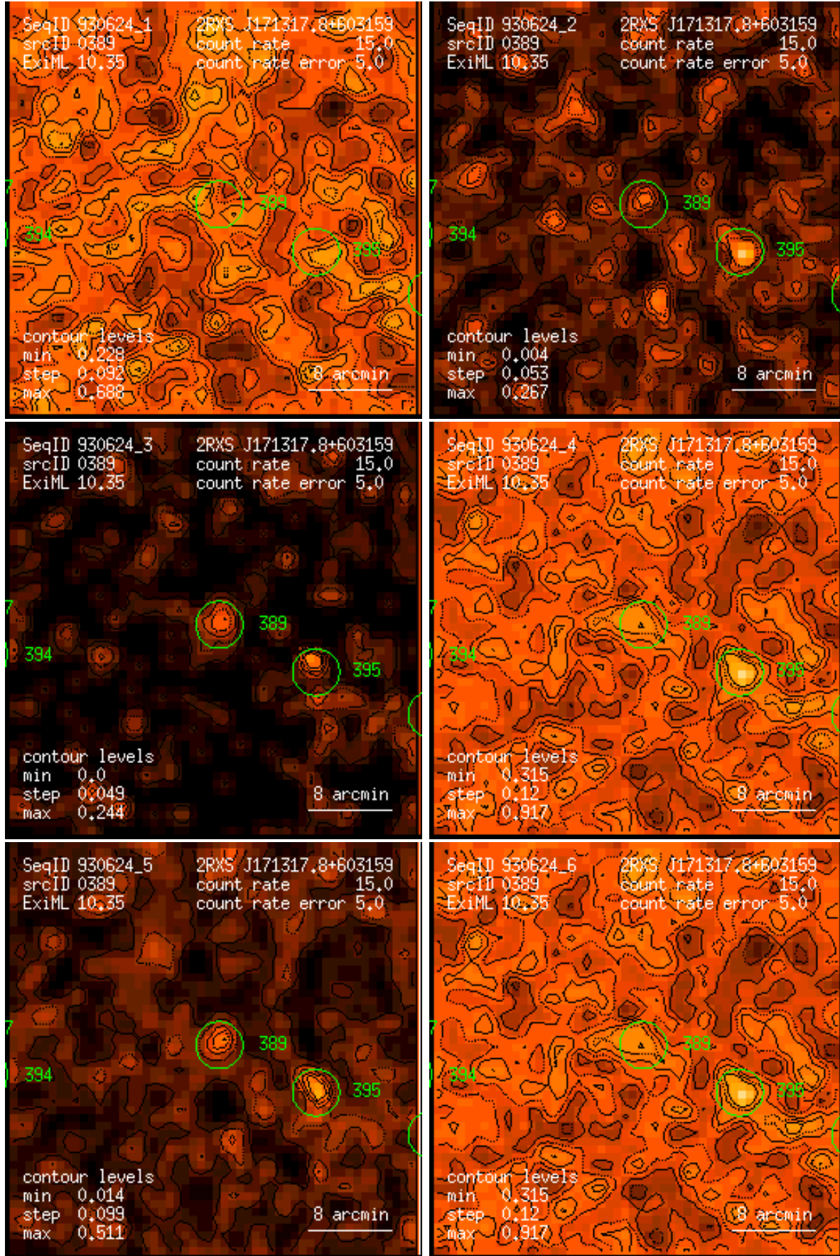
Figure 389: RASS 930624: detection 0389: band rate images, Gaussian filter: (1) PSPC channels 11 – 41, (2) 52 – 90, (3) 91 – 201, (4) 11 – 235, (5) 52 – 201, (6) 11 – 201. Broad band rates in counts/ks. Band rate contour levels in counts/ks/arcmin 2 .
