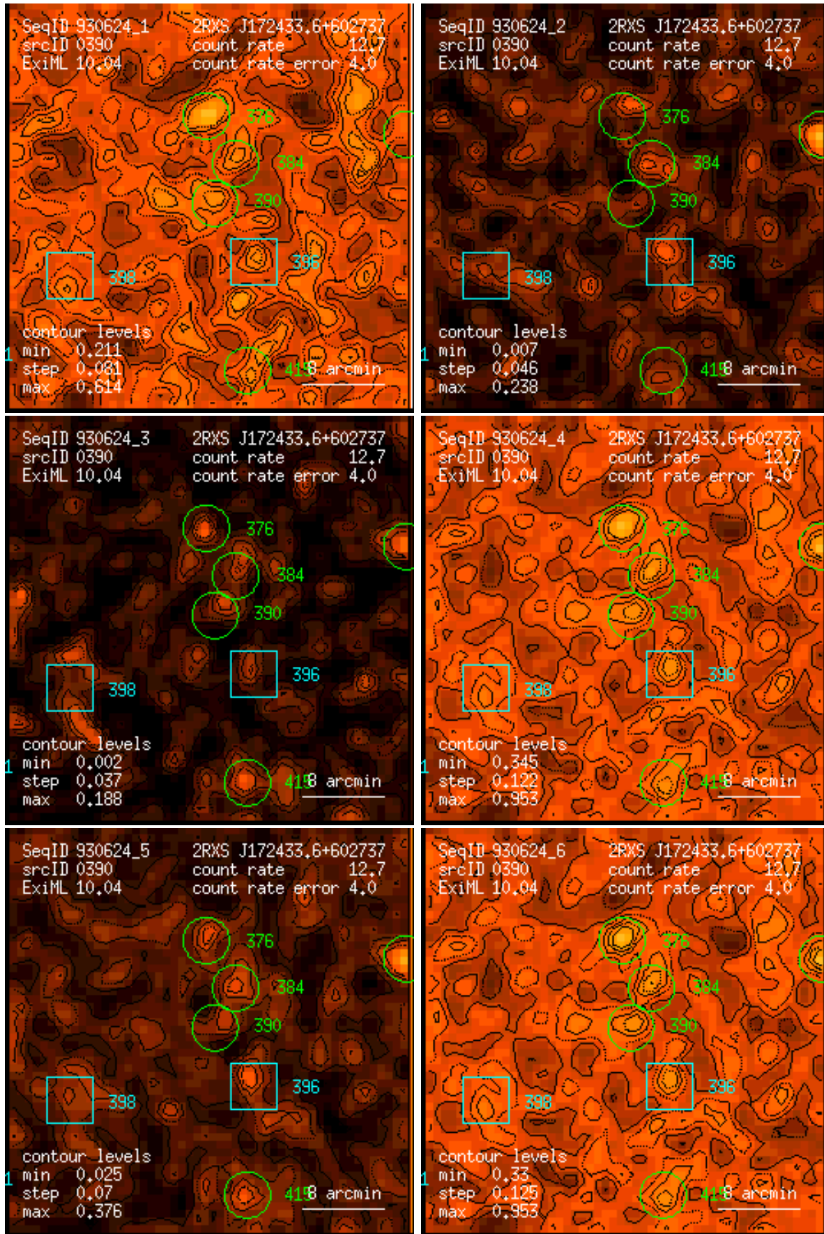
Figure 390: RASS 930624: detection 0390: band rate images, Gaussian filter: (1) PSPC channels 11 – 41, (2) 52 – 90, (3) 91 – 201, (4) 11 – 235, (5) 52 – 201, (6) 11 – 201. Broad band rates in counts/ks. Band rate contour levels in counts/ks/arcmin 2 .
