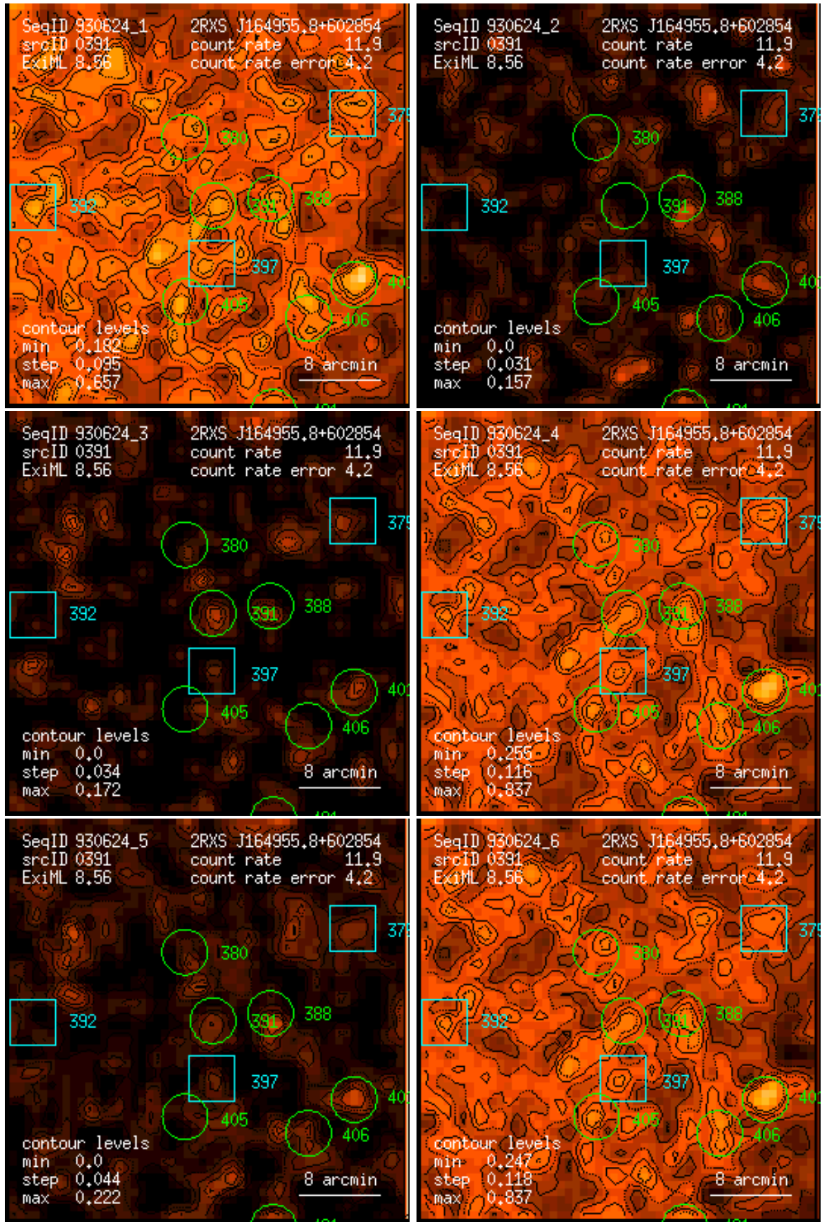
Figure 391: RASS 930624: detection 0391: band rate images, Gaussian filter: (1) PSPC channels 11 – 41, (2) 52 – 90, (3) 91 – 201, (4) 11 – 235, (5) 52 – 201, (6) 11 – 201. Broad band rates in counts/ks. Band rate contour levels in counts/ks/arcmin 2 .
