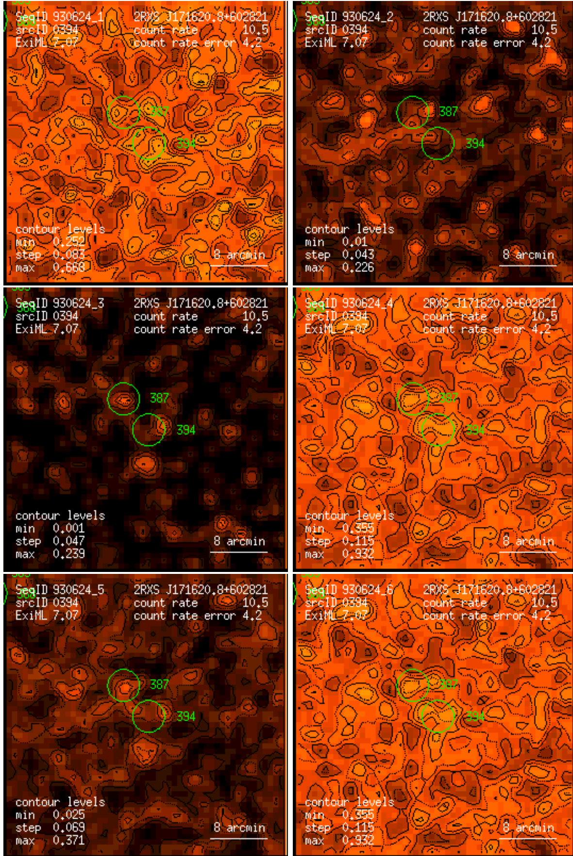
Figure 394: RASS 930624: detection 0394: band rate images, Gaussian filter: (1) PSPC channels 11 – 41, (2) 52 – 90, (3) 91 – 201, (4) 11 – 235, (5) 52 – 201, (6) 11 – 201. Broad band rates in counts/ks. Band rate contour levels in counts/ks/arcmin 2 .
