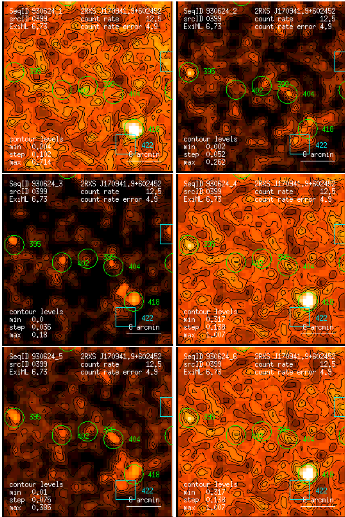
Figure 399: RASS 930624: detection 0399: band rate images, Gaussian filter: (1) PSPC channels 11 – 41, (2) 52 – 90, (3) 91 – 201, (4) 11 – 235, (5) 52 – 201, (6) 11 – 201. Broad band rates in counts/ks. Band rate contour levels in counts/ks/arcmin 2 .
